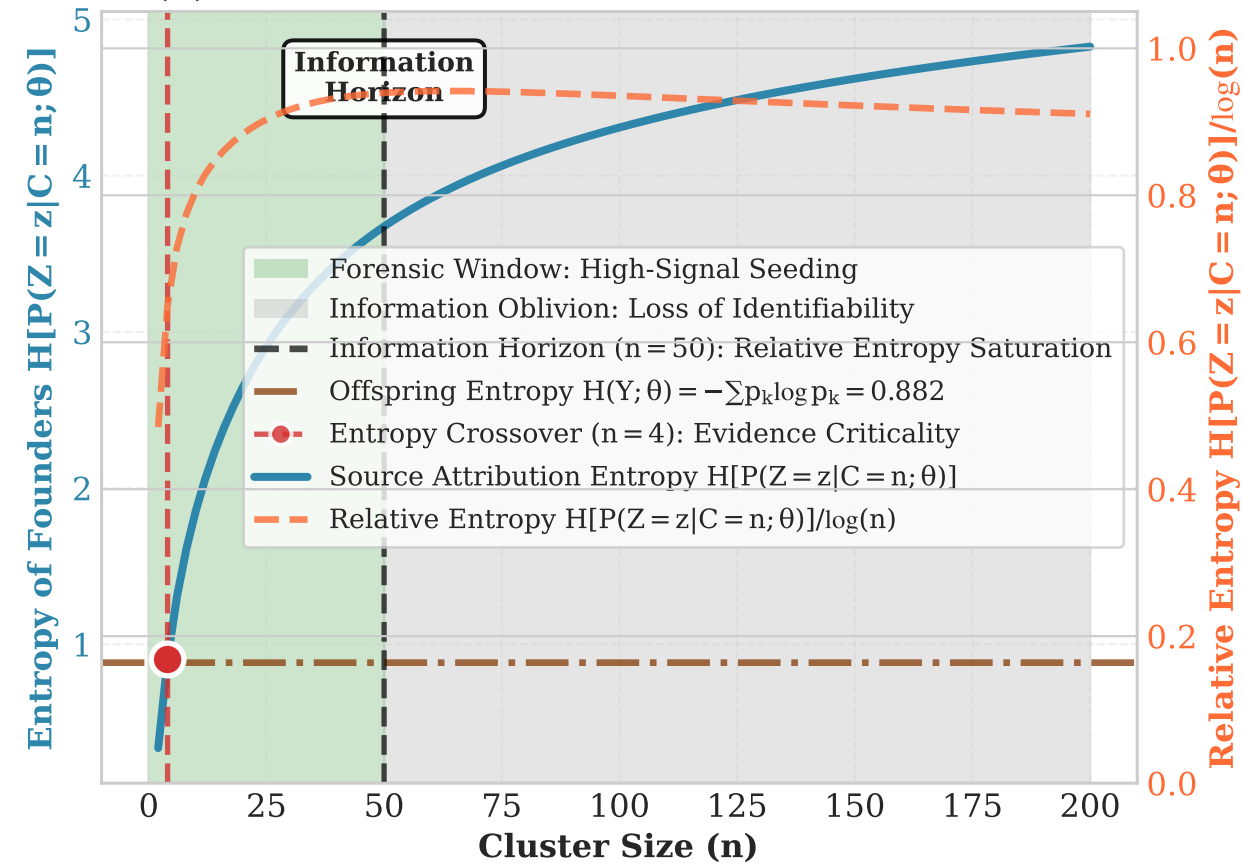
(b) Forensic Information Horizon/Resolution
