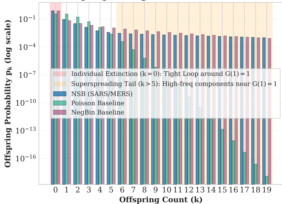
(c) Superspreading Risk & Tail Probabilities
