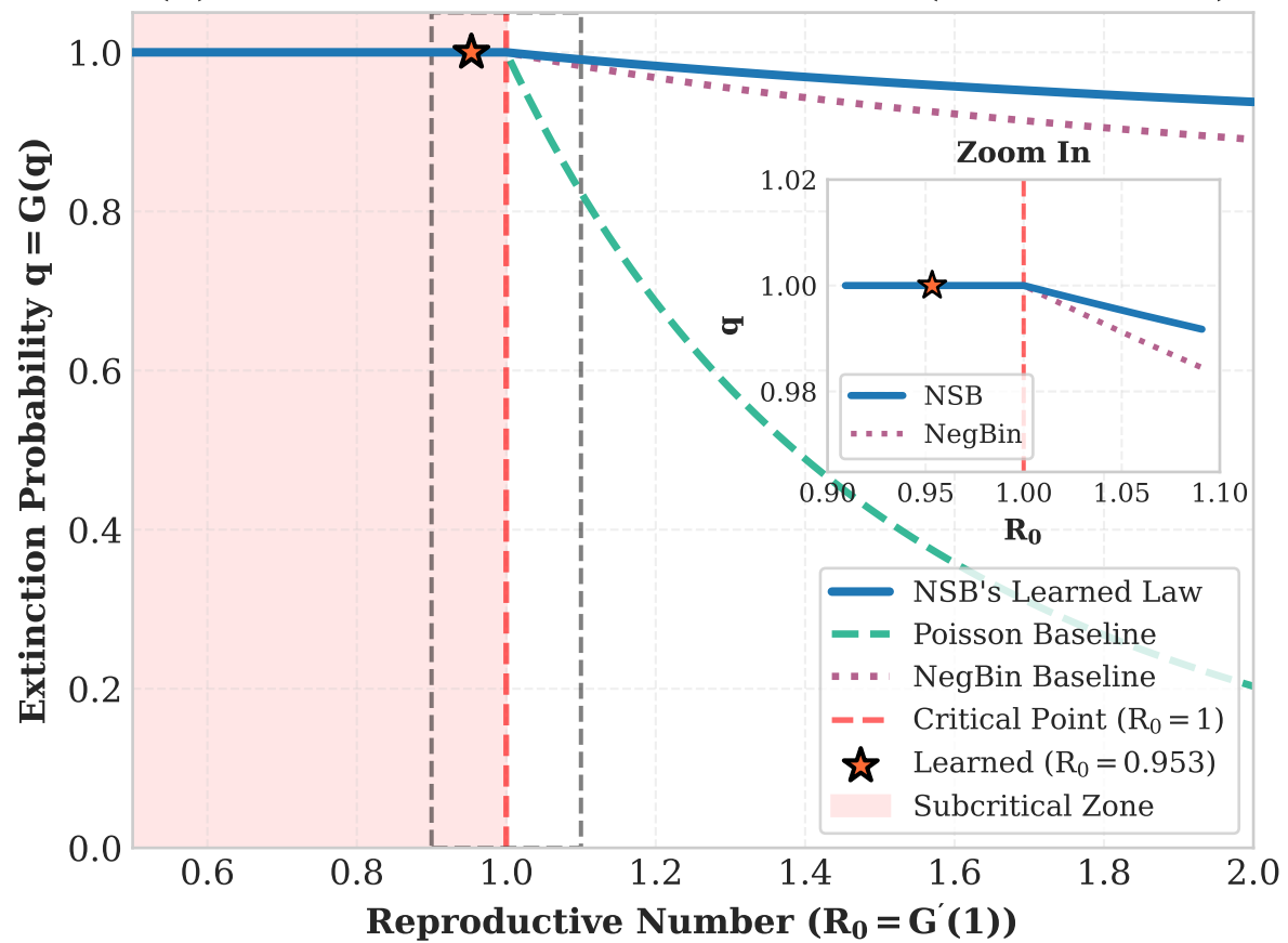
(a) Outbreak Survival Thresholds (SARS/MERS)
