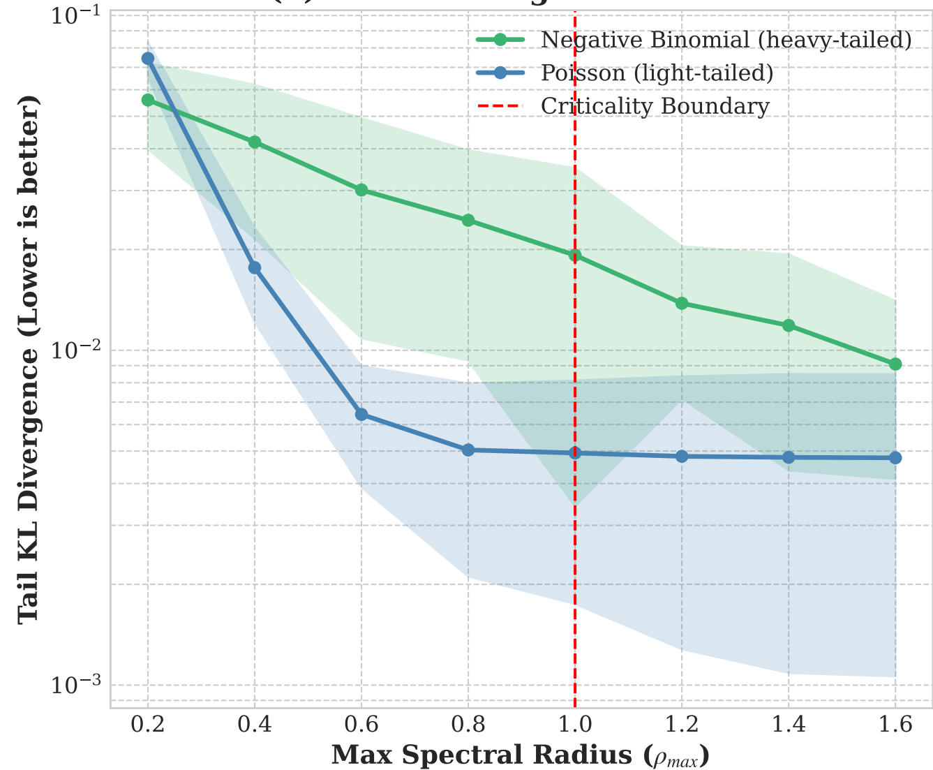
(b) Tail Learning Performance
