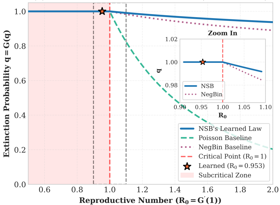
(a) Outbreak Survival Thresholds (SARS/MERS)
