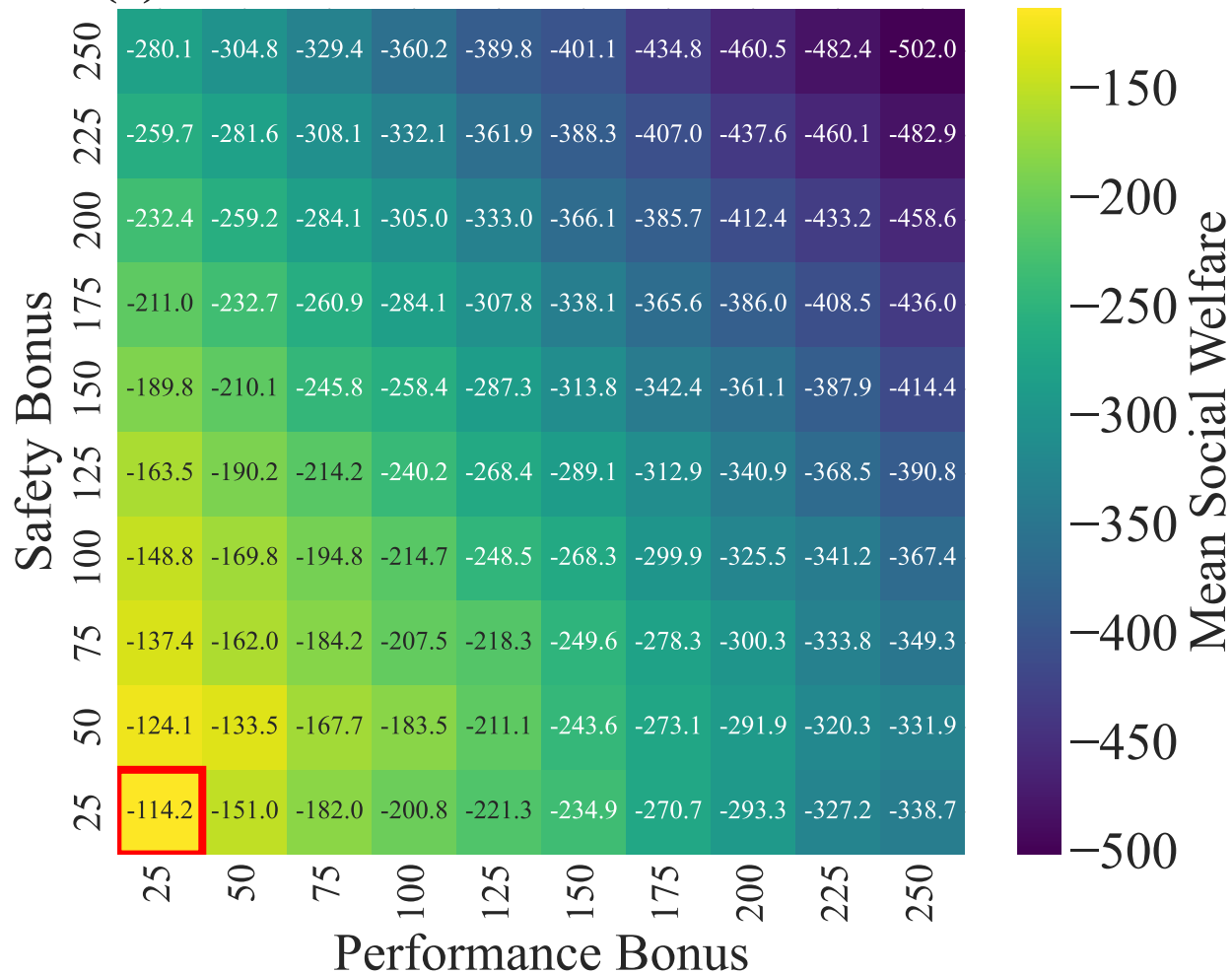
(a) Grid Search for Best-Case Heuristic
