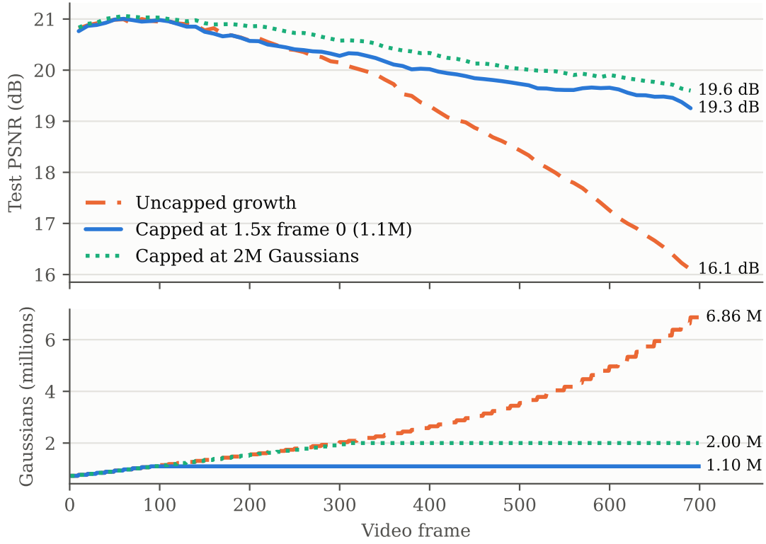
Figure 5: Test PSNR (top) and scene size (bottom) over the video: no cap, a cap at 1.5 times the frame-0 size (1.1 million Gaussians), and a cap at 2 million Gaussians. Setup: RTX PRO 6000 (96 GB); training and test images at 1920 \times 1080 (the 4K capture halved, then undistorted); all 700 frames. Each point is the average over the 24 test cameras.
