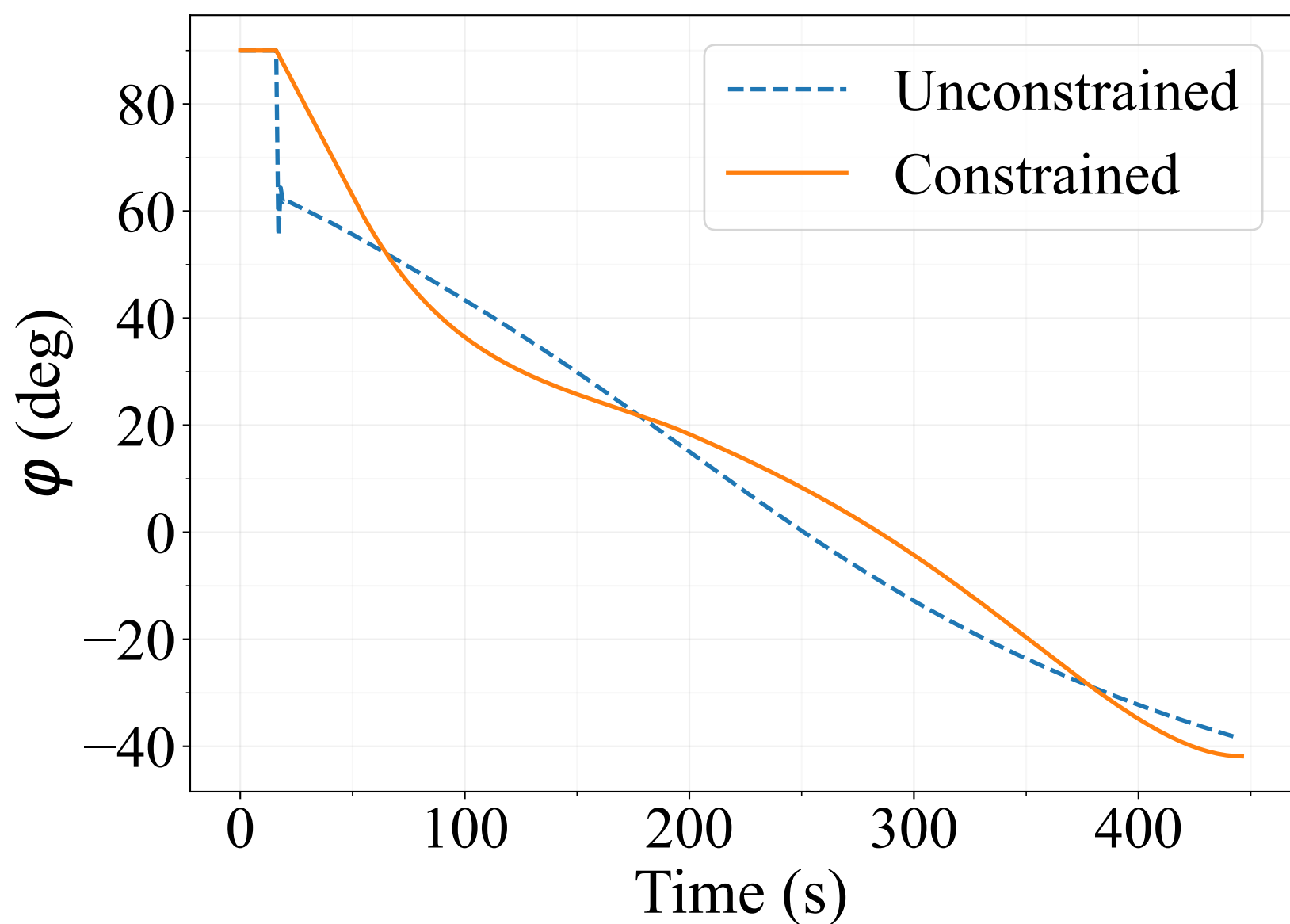
(a) Pitch program angle \varphi
