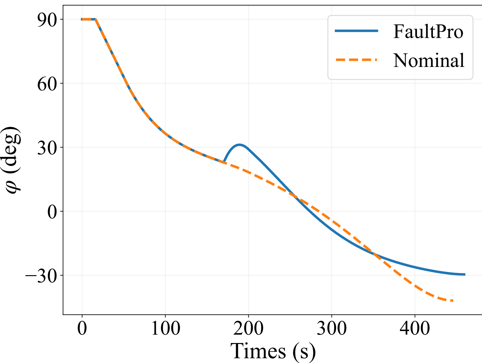
(a) Pitch program angle \varphi
