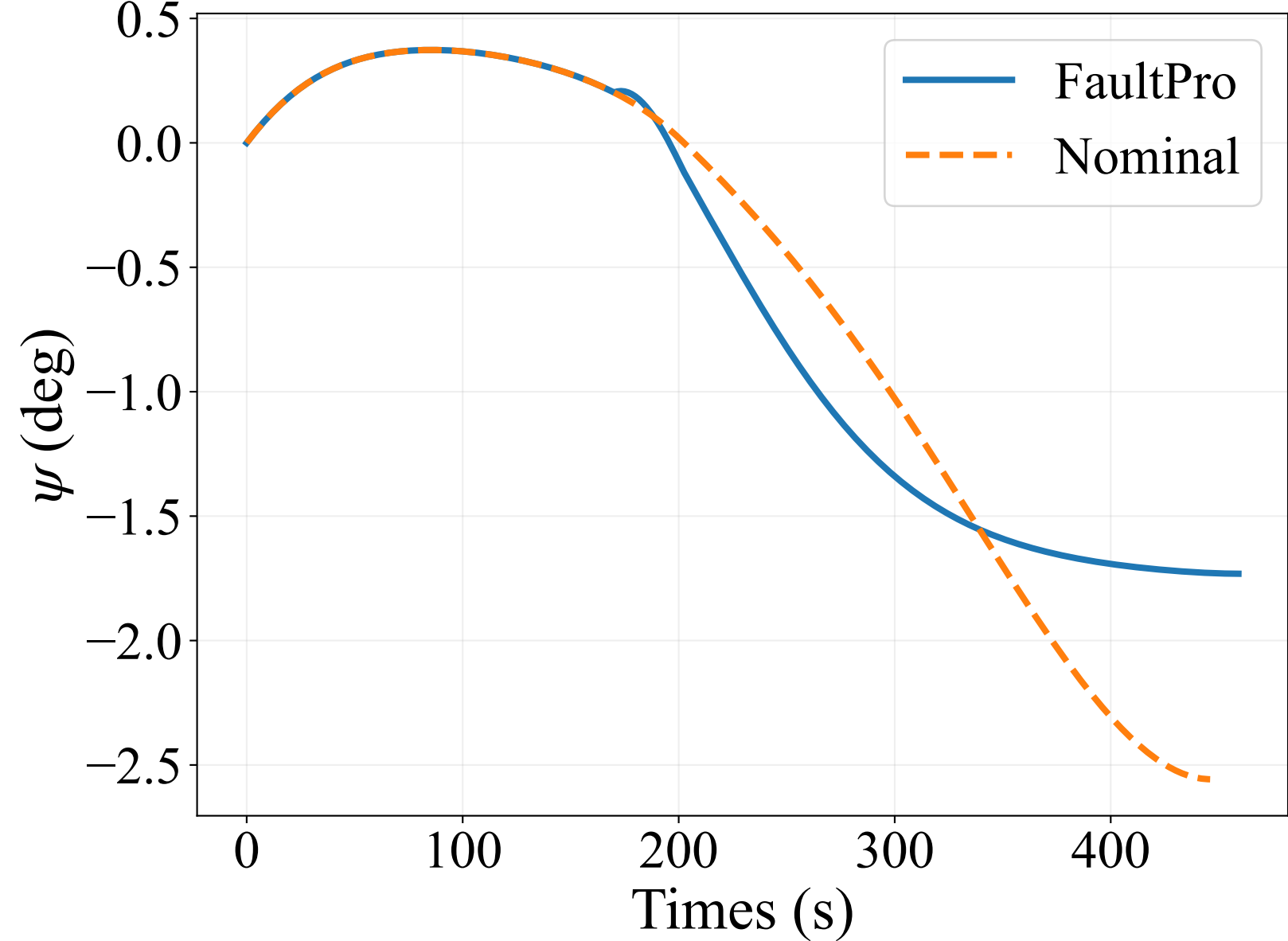
(b) Yaw program angle \psi
