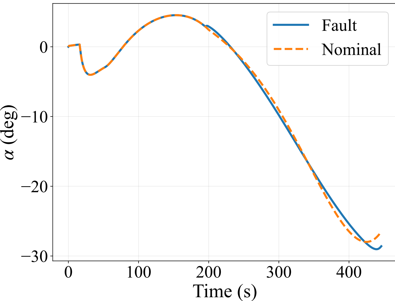
(a) Angle of attack \alpha
