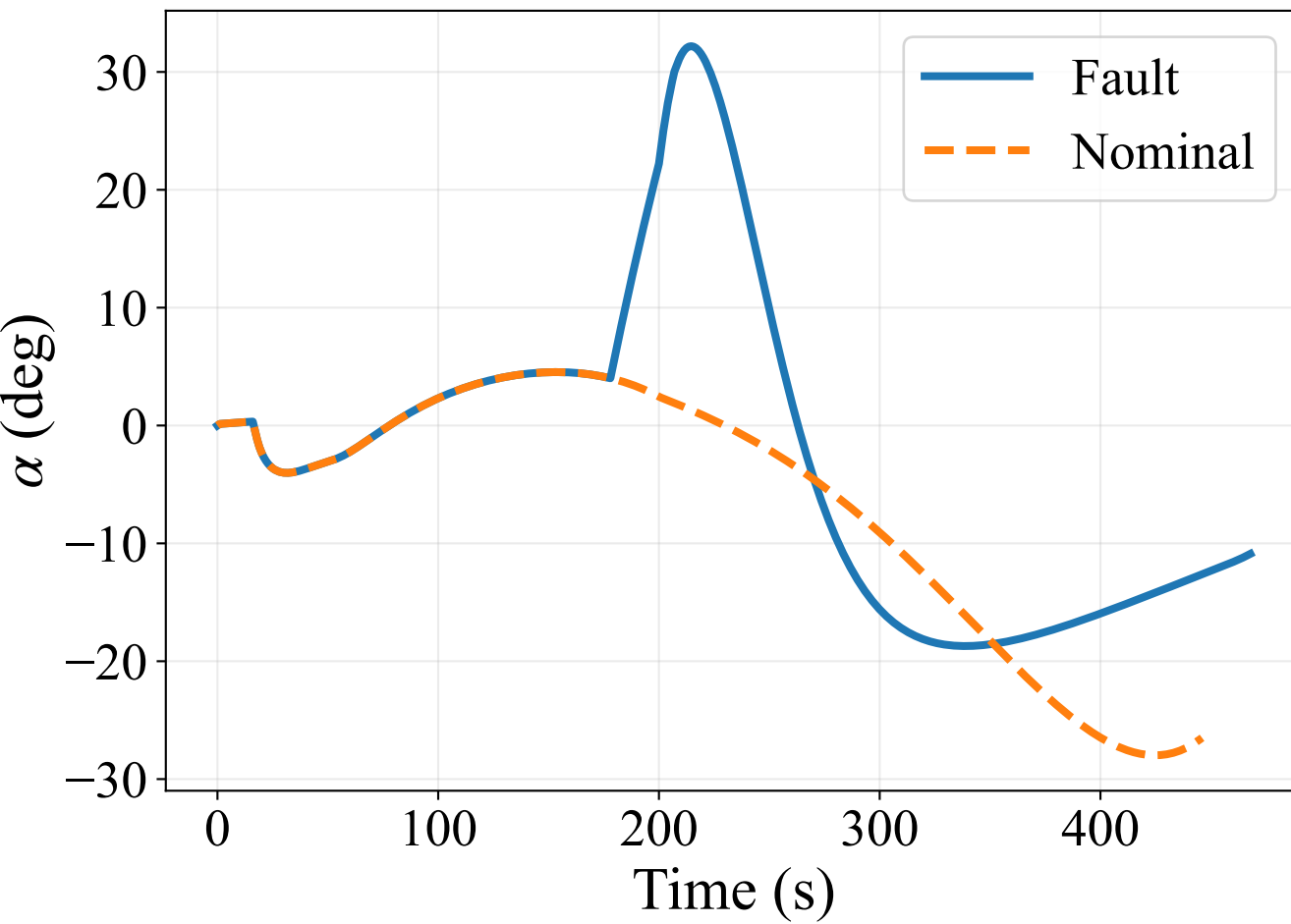
(a) Angle of attack \alpha
