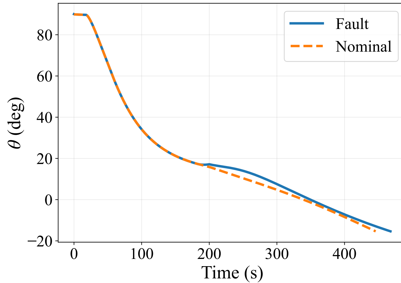
(b) Velocity inclination angle \theta
