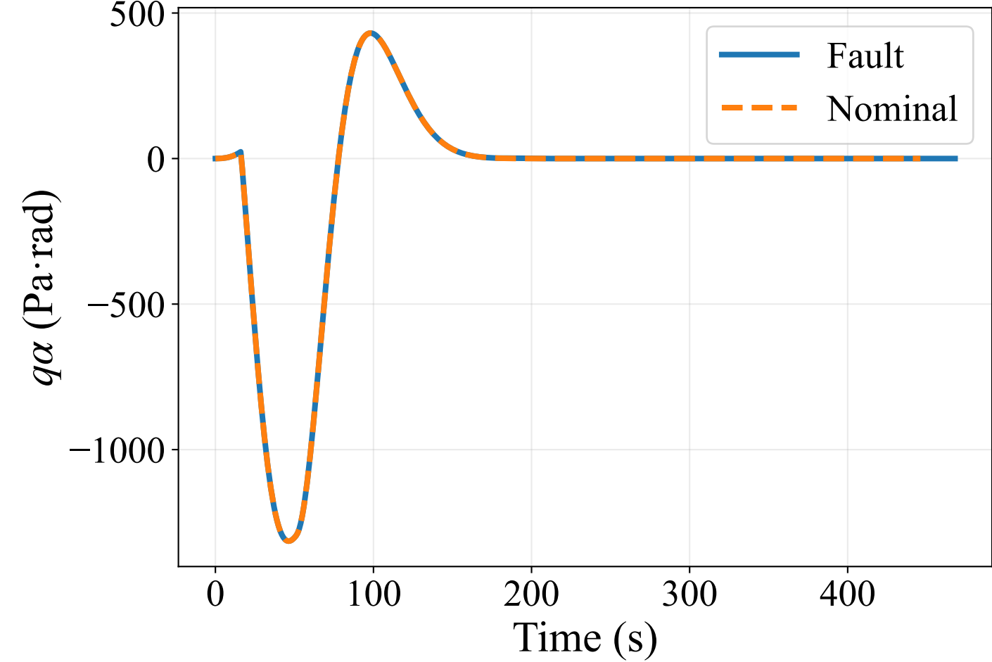
(c) q\alpha load index
