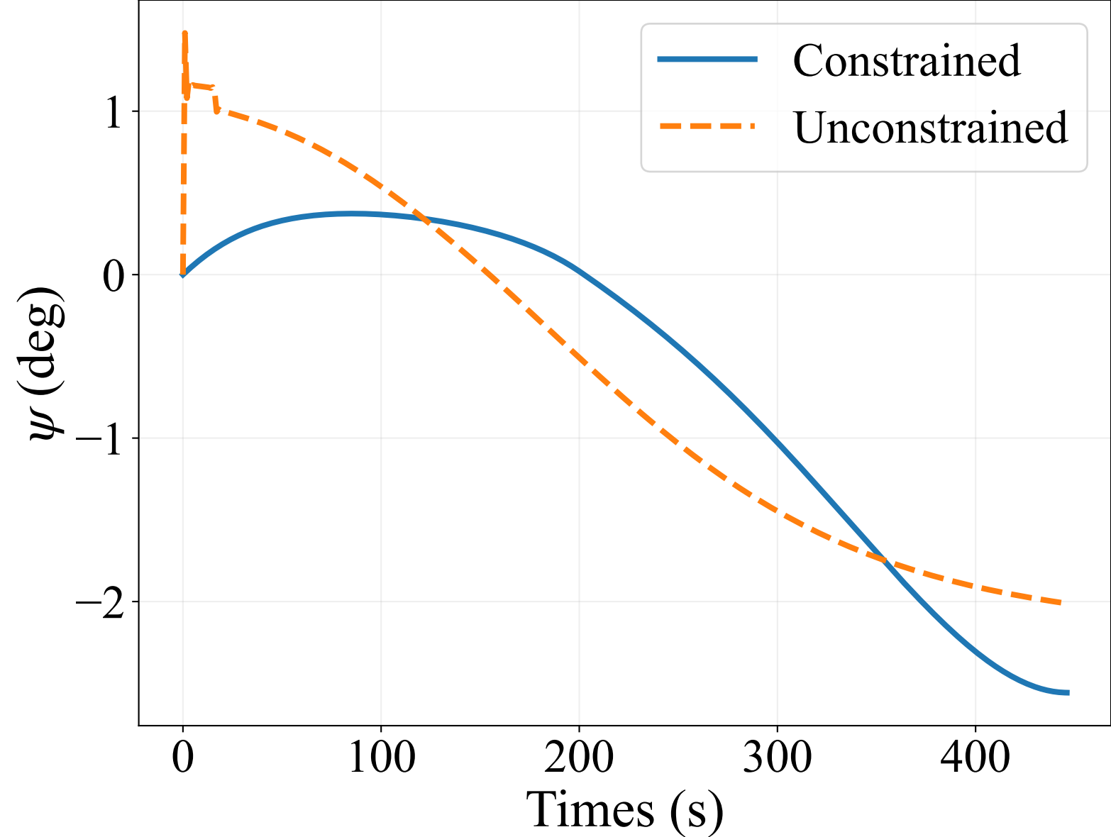
(b) Yaw program angle \psi
