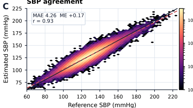
SBP agreement
