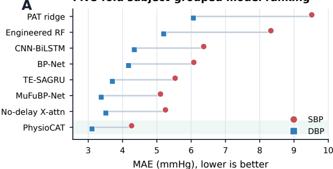
Five-fold subject-grouped model ranking
