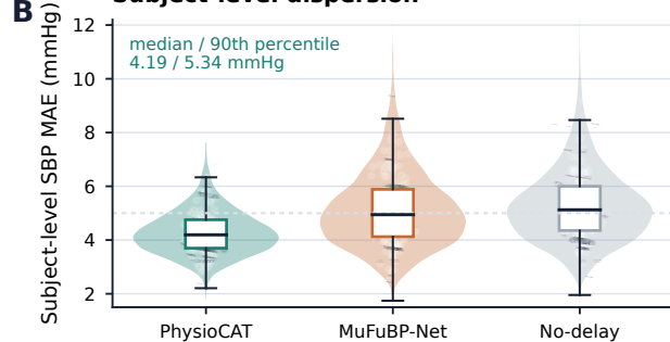
Subject-level dispersion
