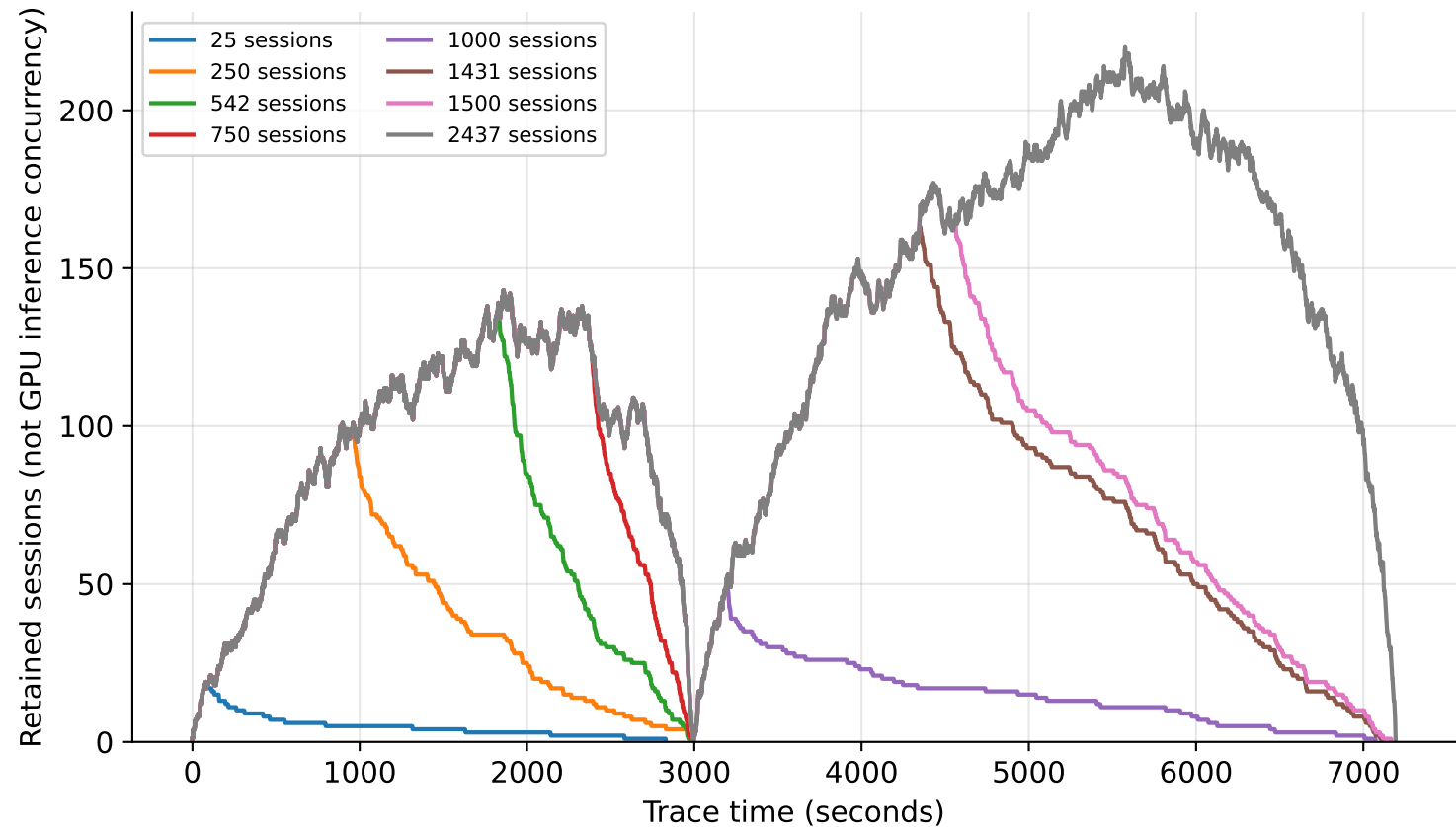
Retained Idle Sessions Over Trace Time
