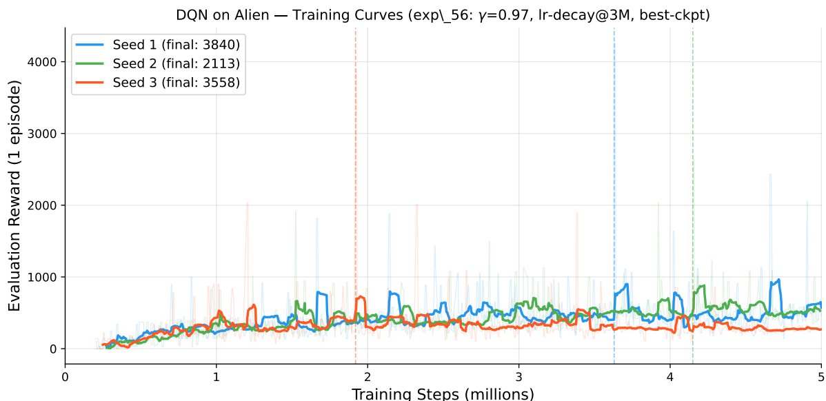
Figure 1: Evaluation reward (1 episode, every 10k steps) for seeds 1, 2, 3. Thin lines are raw; thick lines are a 20-point rolling mean. Dashed vertical lines mark the best-checkpoint step selected for the final 100-episode evaluation.
