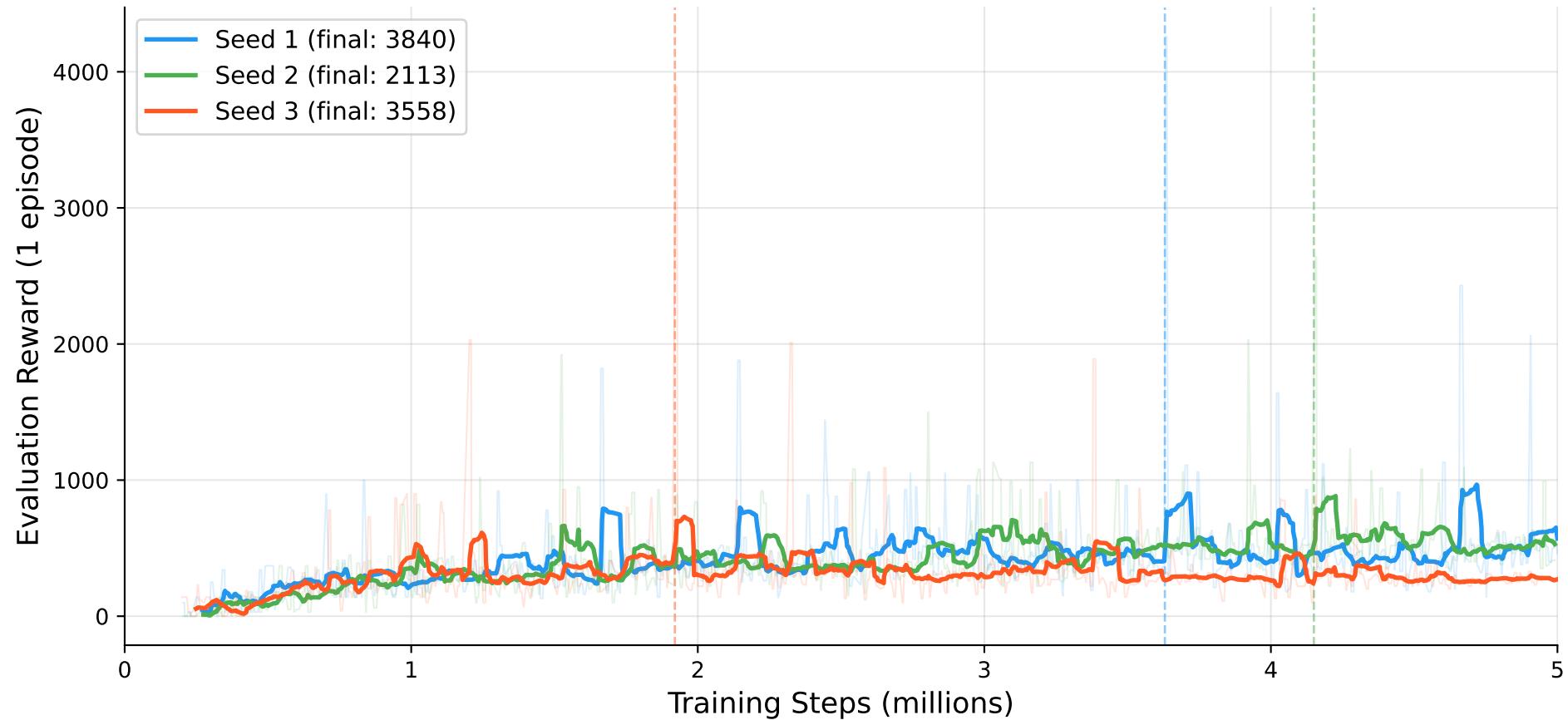
DQN on Alien — Training Curves (exp\_56: \gamma=0.97 , lr-decay@3M, best-ckpt)
