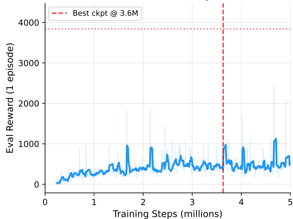
Seed 1 — Final 100-ep: 3840
