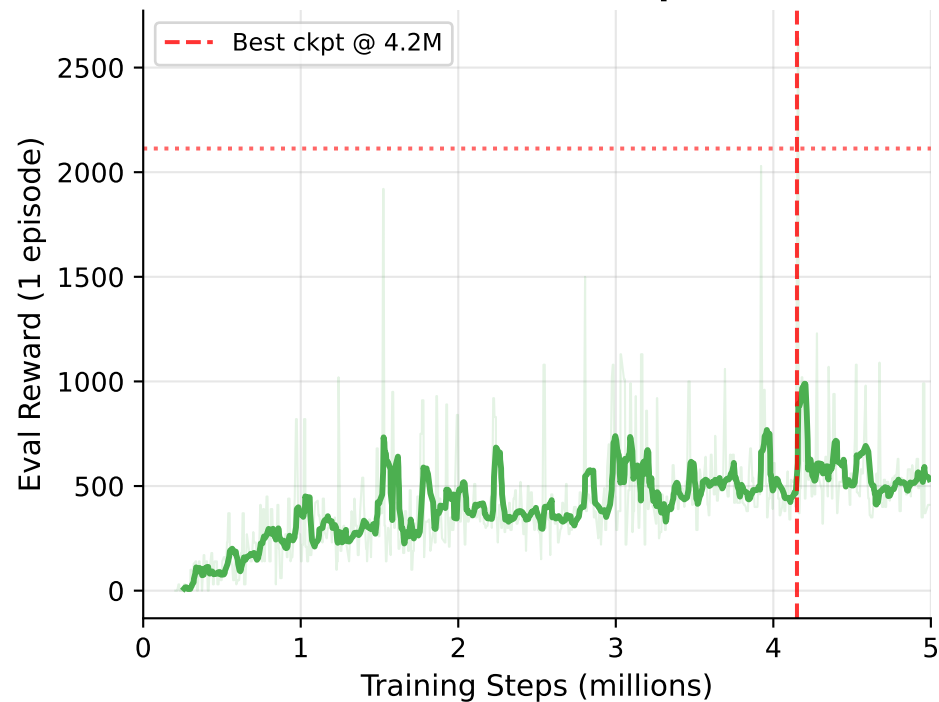
Seed 2 — Final 100-ep: 2113
