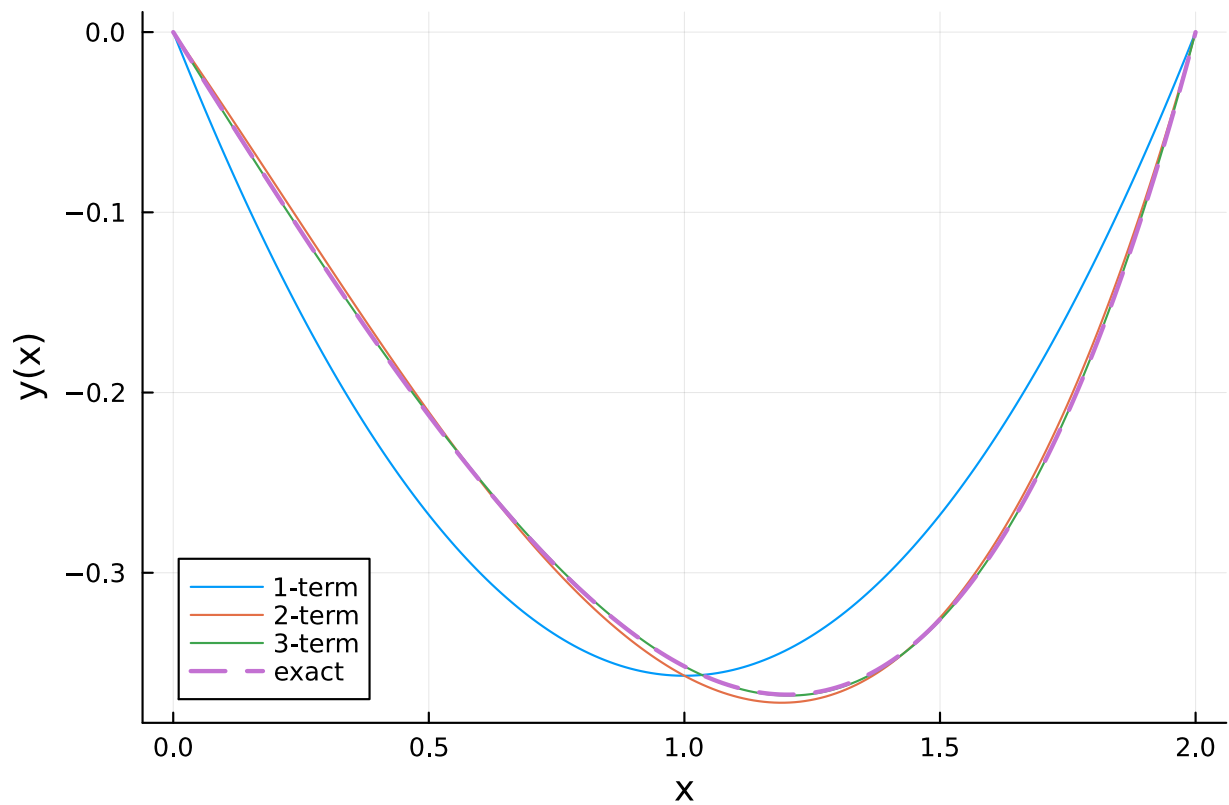
Figure 3: Ritz Approximations
