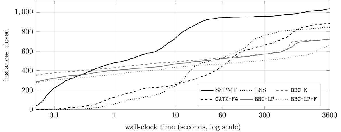
Figure 10: Every solved run in the campaign, not the six sampled columns of Table 7: for each method, the number of instances closed by each wall-clock time. The curves cross, and where they cross is what matters here. Before about two seconds the configurations built here lead the field — BBC-K has a median solve time of 0.06 seconds against 59.8 for CATZ-F4 — because a Benders master with a tight coverage row closes an instance at the root immediately or not at all. After two seconds they stop moving and every compact model overtakes them. The decomposition is not running out of time. It has stopped making progress, and what would restart it is a bound that improves when the solver branches.
