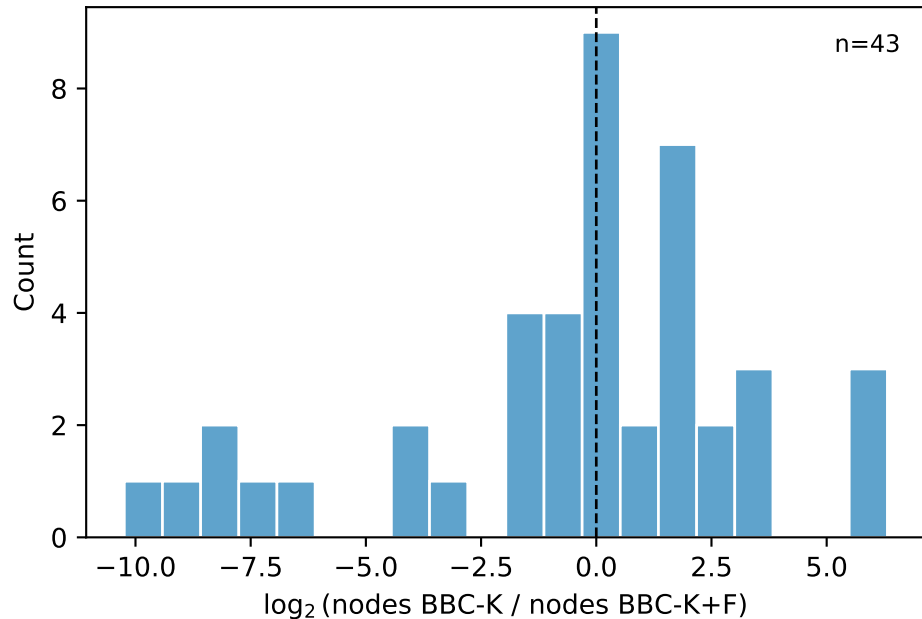
Node reduction from fractional cuts [ J \leq 10 ]
