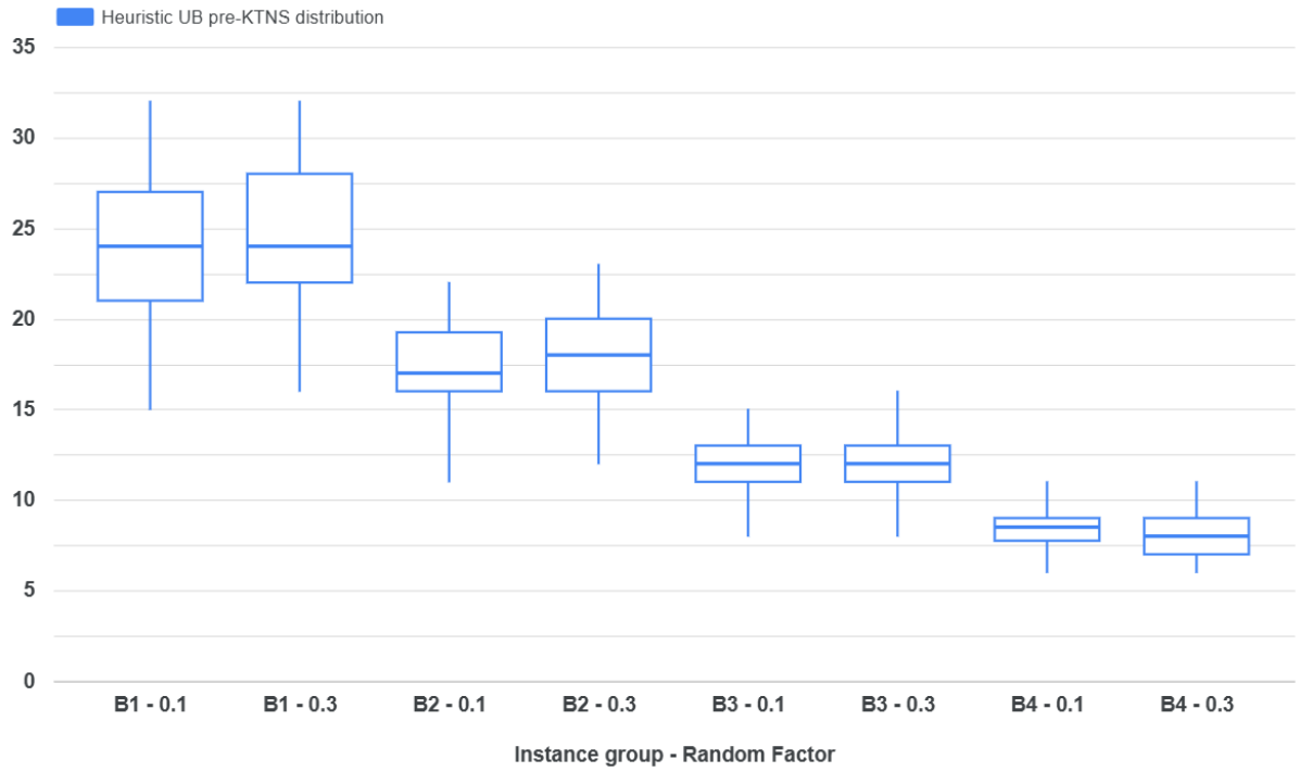
Figure 4.16: Box plot of the obtained upper bound values before applying the KTNS policy for each subgroup of instances of datB and each value of Random Factor.
