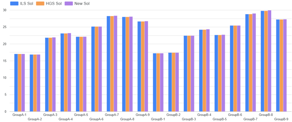
Figure 4.9: Obtained upper bounds with ILS, HGS and New Heuristics for every instance from Yanasse dataset Yanasse et al. (2009) for GroupA and GroupB.
