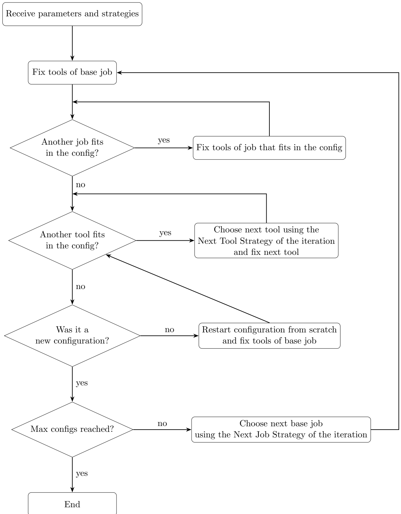
Figure 3.4: Flow diagram describing the extra configuration creation process of a multi-start run in the heuristic method.
