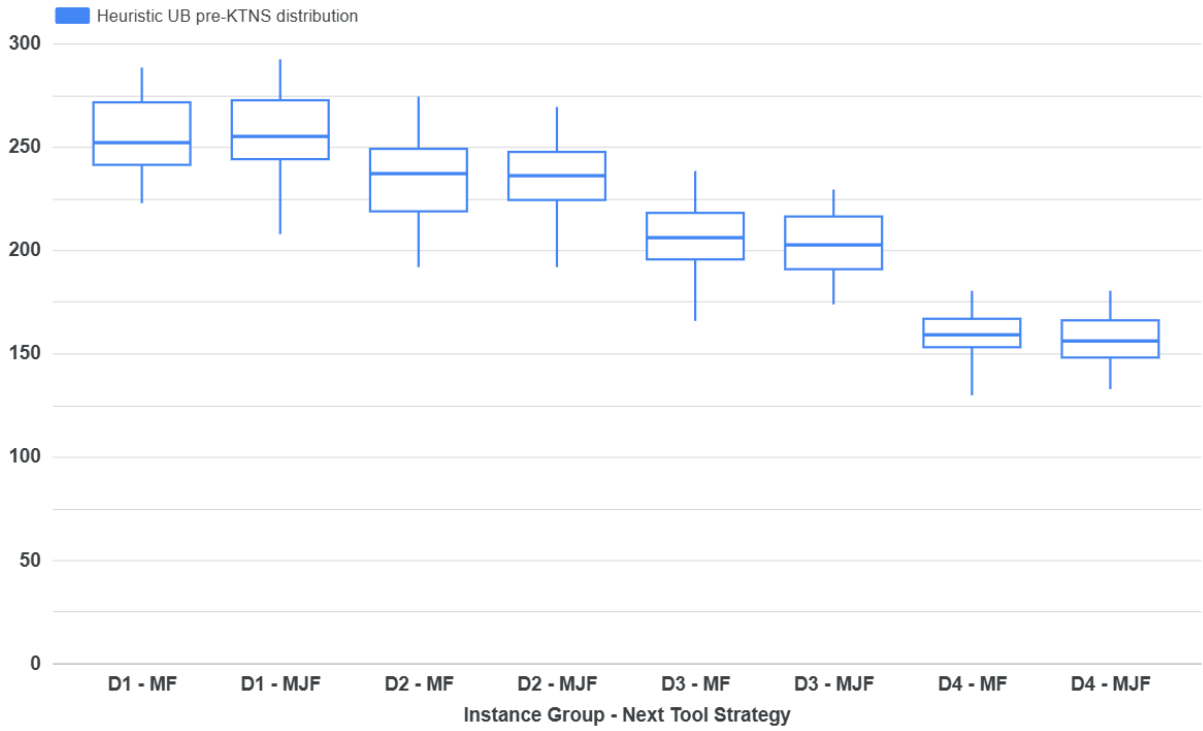
Figure 4.22: Box plot of the obtained upper bound values before applying the KTNS policy for each subgroup of instances of datD and each option of Next Tool Strategy.
