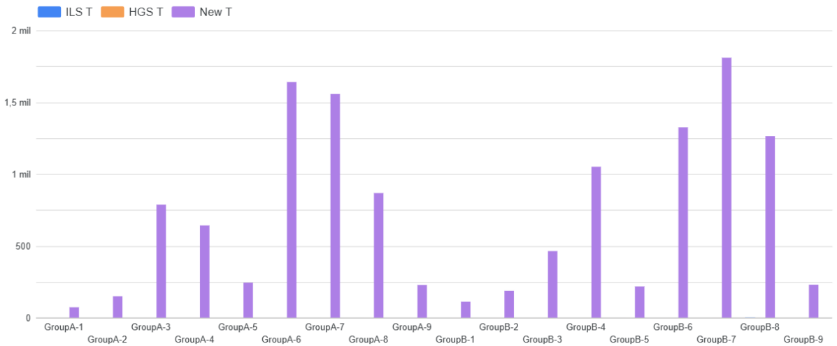
Figure 4.10: Time in seconds with ILS, HGS and New Heuristics to obtain the upper bound for every instance from Yanasse dataset Yanasse et al. (2009) for GroupA and GroupB.
