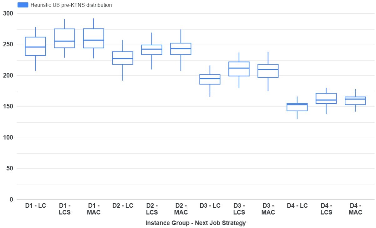
Figure 4.26: Box plot of the obtained upper bound values before applying the KTNS policy for each subgroup of instances of datD and each option of Next Job Strategy.
