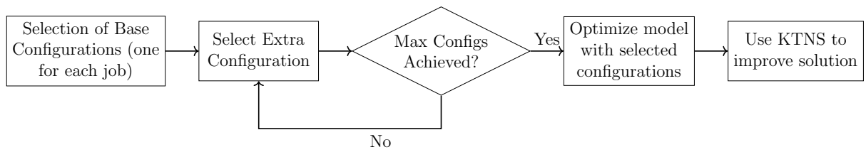
Figure 3.5: Flow diagram describing the configuration selection in the mixing and improving phase.
