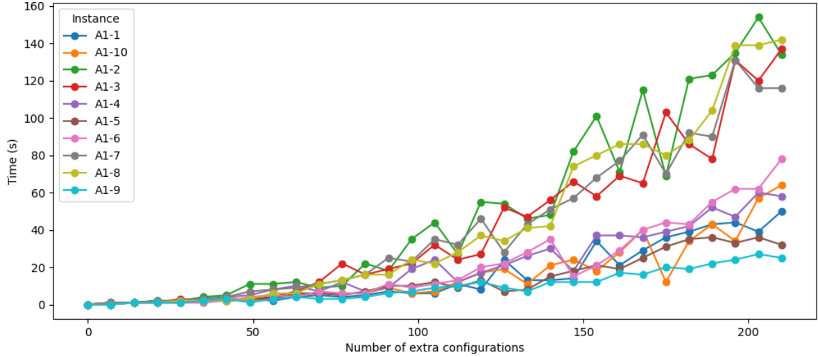
Figure 3.1: Computational time (s) to solve new formulation for 10 small instances by number of extra configurations provided.
