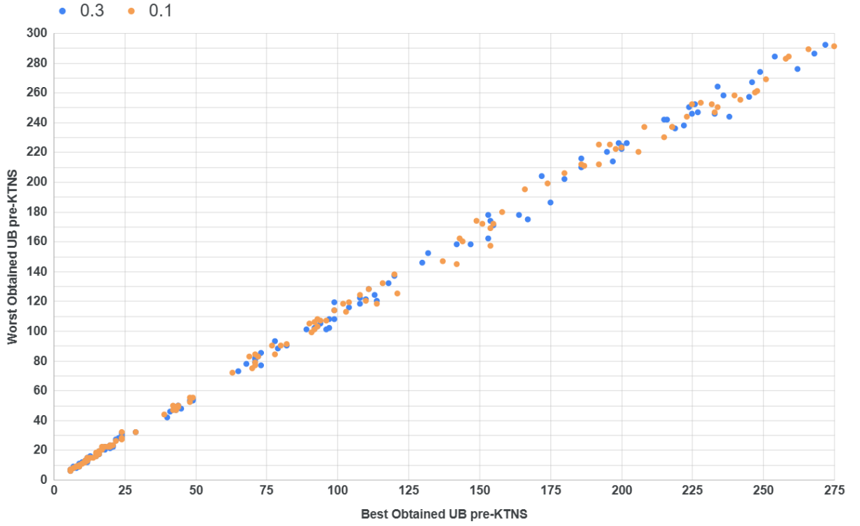
Figure 4.15: Distribution of instances for best obtained upper bound before applying KTNS and worst obtained upper bound before applying KTNS for each multi-start run, both in number of switches, separating for Random Factor used in the run.
