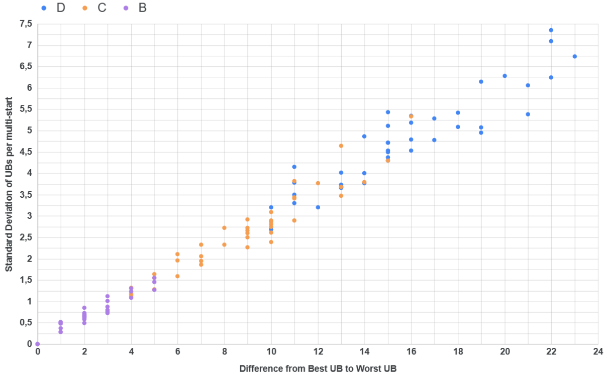
Figure 4.1: Distribution of instances for best to worst solution gap by standard deviation of obtained solutions.
