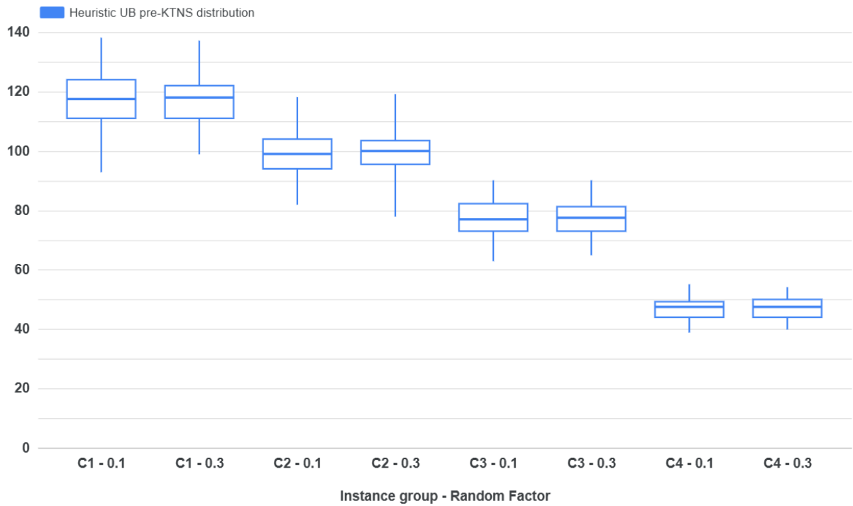
Figure 4.17: Box plot of the obtained upper bound values before applying the KTNS policy for each subgroup of instances of datC and each value of Random Factor.
