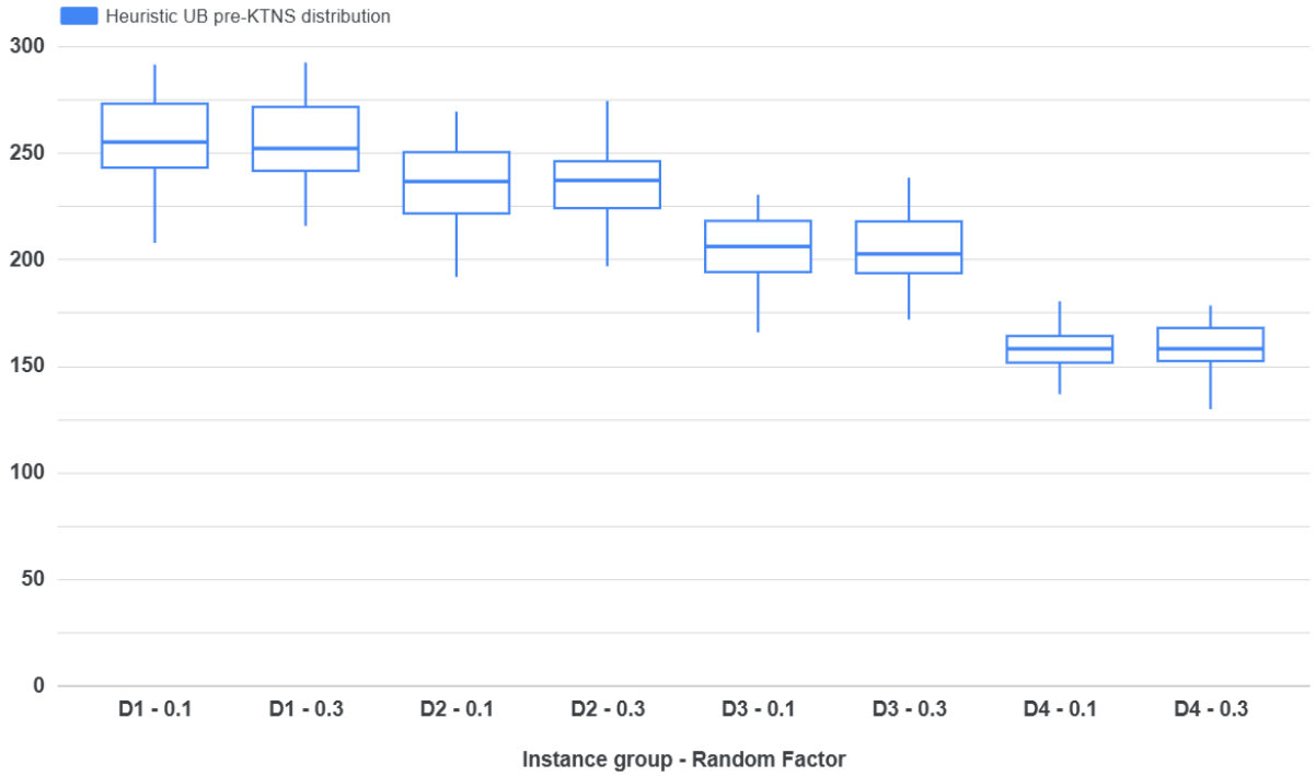
Figure 4.18: Box plot of the obtained upper bound values before applying the KTNS policy for each subgroup of instances of datD and each value of Random Factor.
