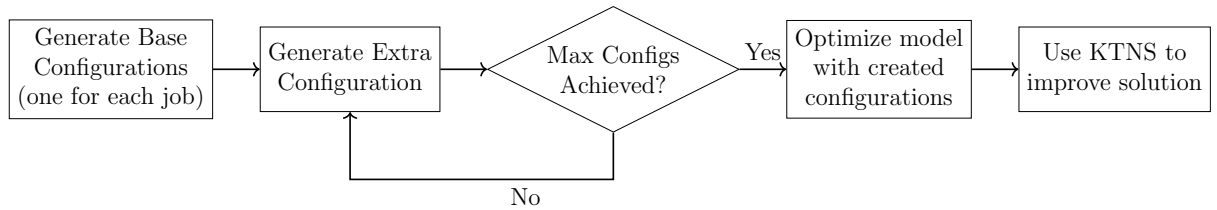
Figure 3.2: Flow diagram describing the multi-start configuration generation phase.
