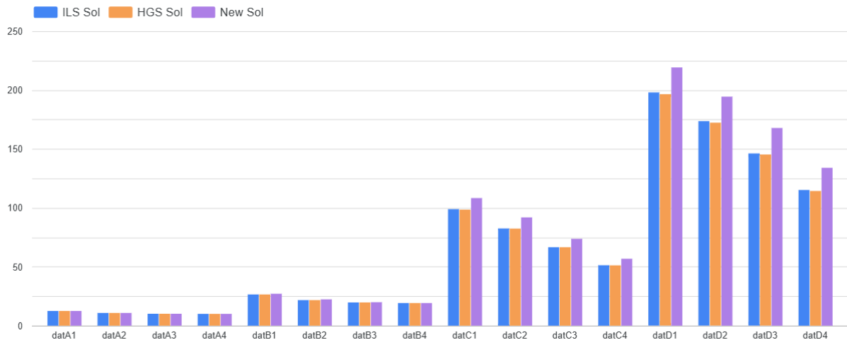
Figure 4.5: Obtained upper bounds with ILS, HGS and New Heuristics for every instance from Catanzaro dataset Catanzaro et al. (2015) .
