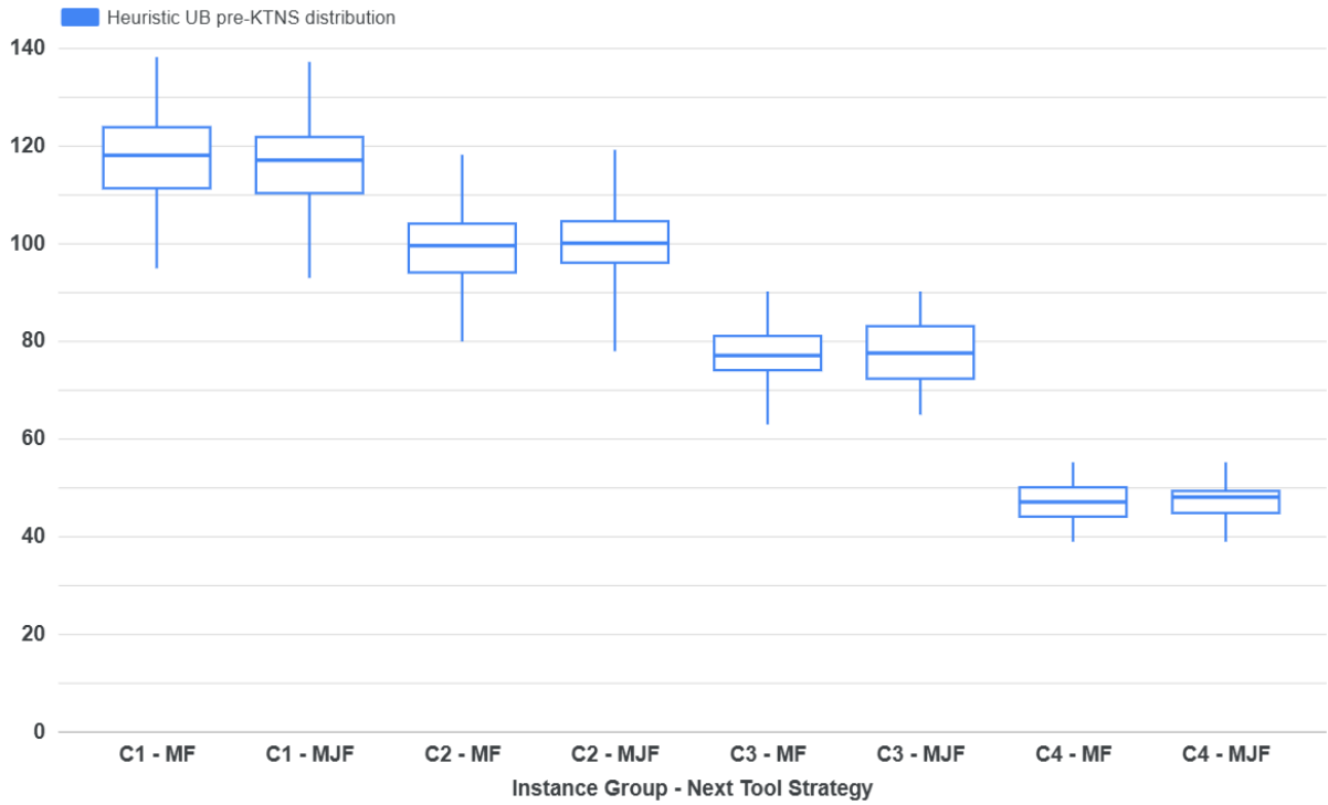
Figure 4.21: Box plot of the obtained upper bound values before applying the KTNS policy for each subgroup of instances of datC and each option of Next Tool Strategy.
