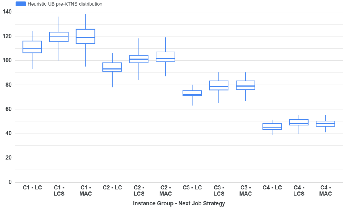
Figure 4.25: Box plot of the obtained upper bound values before applying the KTNS policy for each subgroup of instances of datC and each option of Next Job Strategy.
