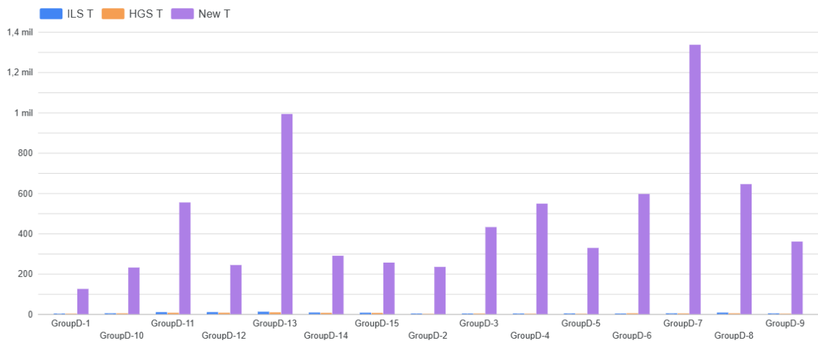
Figure 4.14: Time in seconds with ILS, HGS and New Heuristics to obtain the upper bound for every instance from Yanasse dataset Yanasse et al. (2009) for GroupD.
