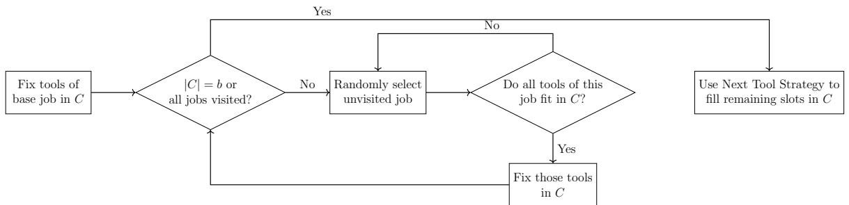
Figure 3.3: Flow diagram describing the multi-job configuration creator.
