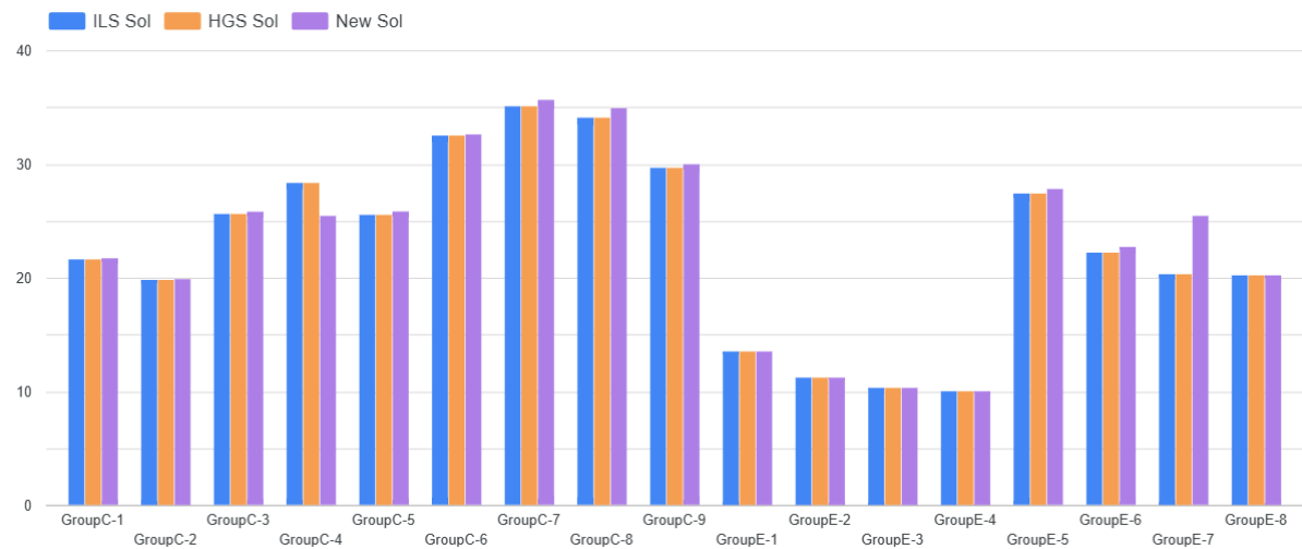
Figure 4.11: Obtained upper bounds with ILS, HGS and New Heuristics for every instance from Yanasse dataset Yanasse et al. (2009) for GroupC and GroupE.
