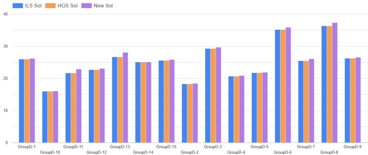
Figure 4.13: Obtained upper bounds with ILS, HGS and New Heuristics for every instance from Yanasse dataset Yanasse et al. (2009) for GroupD.
