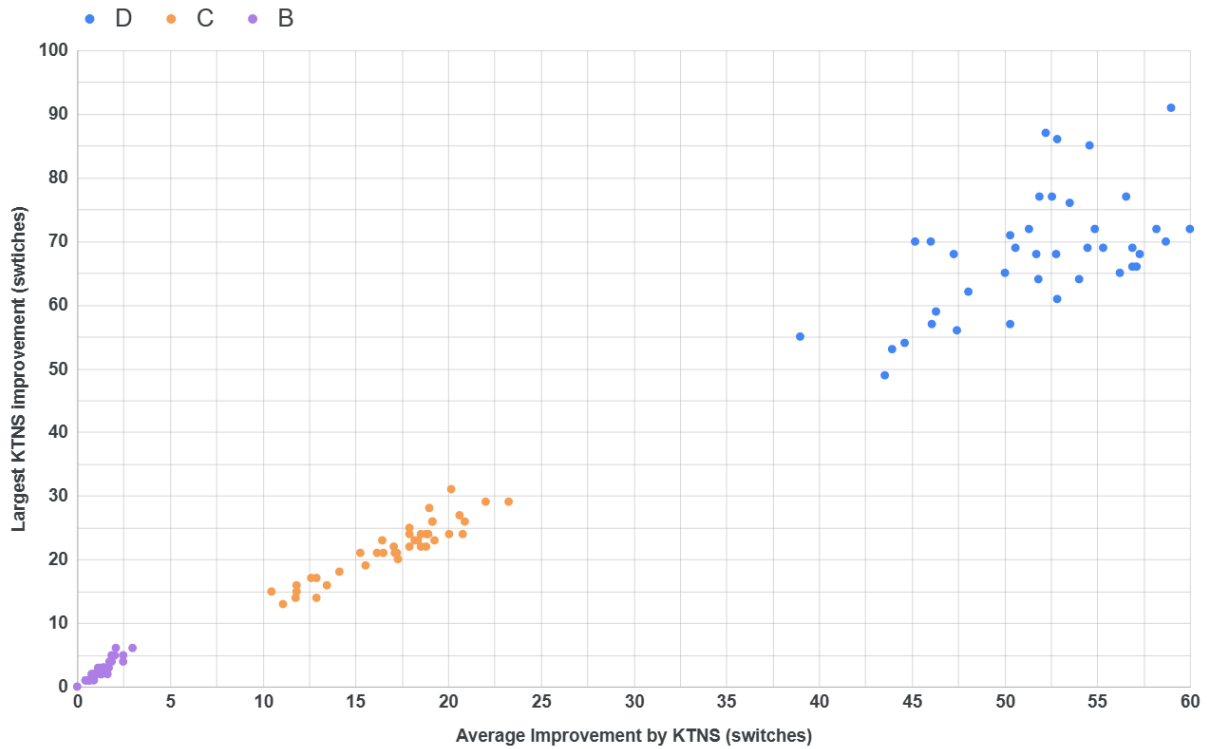
Figure 4.3: Distribution of instances for Average Improvement by applying KTNS by Largest Improvement by applying KTNS, both in number of switches reduced.
