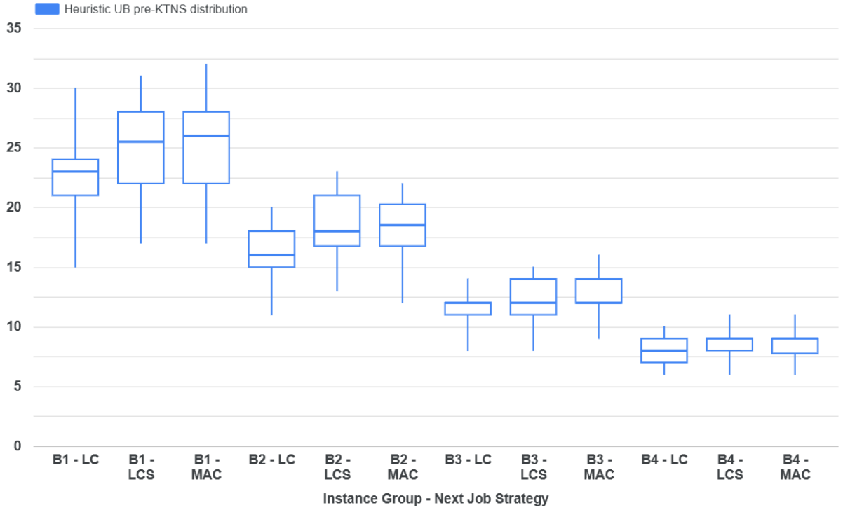
Figure 4.24: Box plot of the obtained upper bound values before applying the KTNS policy for each subgroup of instances of datB and each option of Next Job Strategy.
