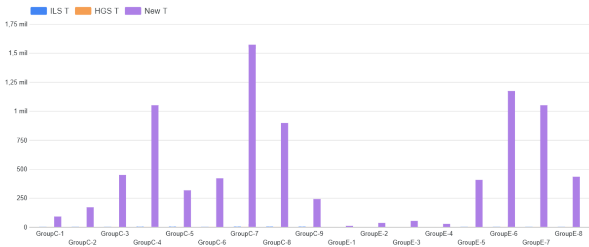
Figure 4.12: Time in seconds with ILS, HGS and New Heuristics to obtain the upper bound for every instance from Yanasse dataset Yanasse et al. (2009) for GroupC and GroupE.
