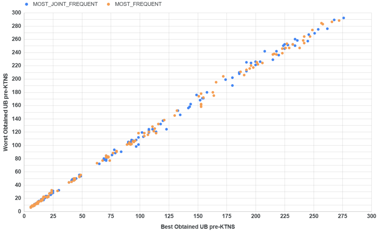
Figure 4.19: Distribution of instances for best obtained upper bound before applying KTNS and worst obtained upper bound before applying KTNS for each multi-start run, both in number of switches, separating for Next Tool Strategy used in the run.
