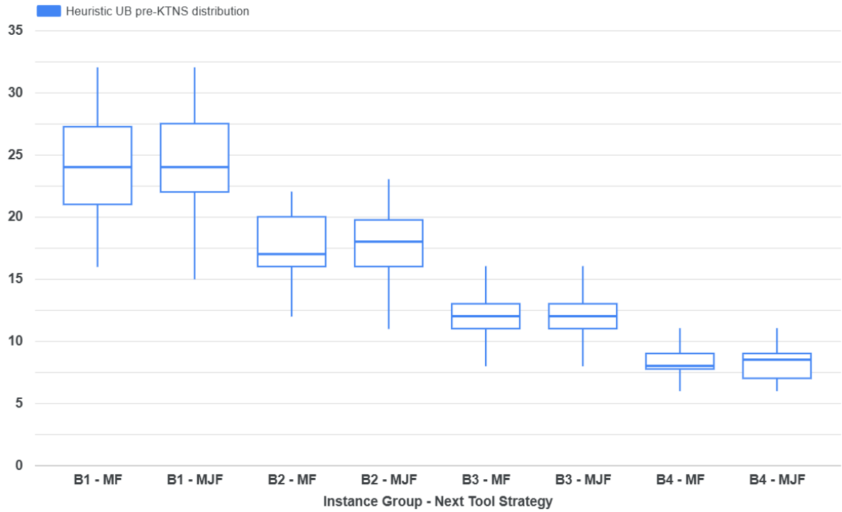
Figure 4.20: Box plot of the obtained upper bound values before applying the KTNS policy for each subgroup of instances of datB and each option of Next Tool Strategy.
