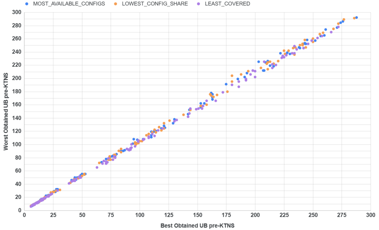
Figure 4.23: Distribution of instances for best obtained upper bound before applying KTNS and worst obtained upper bound before applying KTNS for each multi-start run, both in number of switches, separating for Next Job Strategy used in the run.
