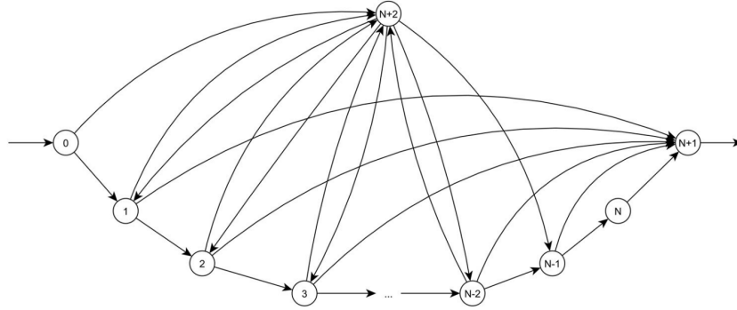
Figure 1.1: Directed graph for SSPMF from da Silva et al. (2021)
