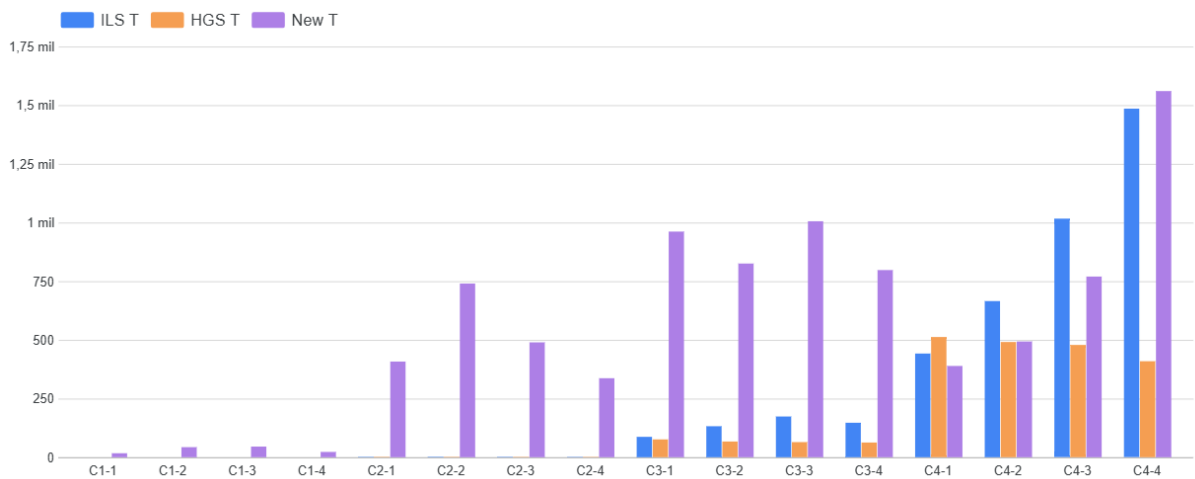
Figure 4.8: Time in seconds with ILS, HGS and New Heuristics to obtain the upper bound for every instance from Crama dataset Crama (1997) .
