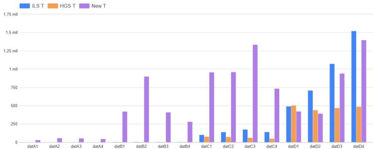
Figure 4.6: Time in seconds with ILS, HGS and New Heuristics to obtain the upper bound for every instance from Catanzaro dataset Catanzaro et al. (2015) .
