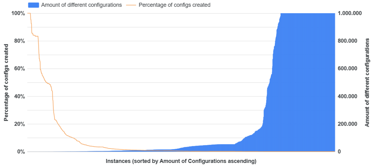
Figure 4.4: Amount of different configurations and percentage of configurations that 100 configurations mean for each instance in all three data sets.
