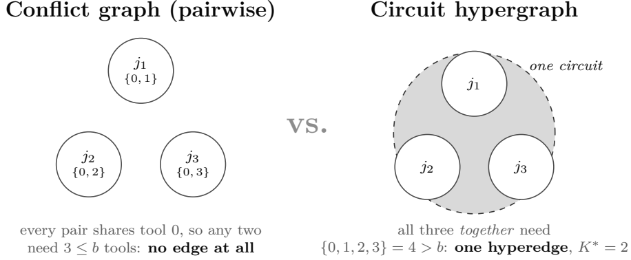
Figure 9: The circuit hypergraph, on the star instance T_1 = \{0, 1\} , T_2 = \{0, 2\} , T_3 = \{0, 3\} with b = 3 . No two jobs conflict—each pair needs only three tools, which fit—so the conflict graph has no edges at all. Yet all three together need four tools and overflow the magazine: \{j_1, j_2, j_3\} is a circuit , a minimal infeasible set, drawn here as the shaded hyperedge that no graph of pairwise conflicts can express. It already forces K^* = 2 . This is exactly why K^* is read off the hypergraph of all minimal clashes (Proposition 11), never the graph of pairwise ones alone.
