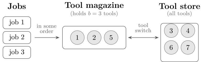
Figure 1: The physical setting. A computer-controlled machine draws tools from a magazine that holds only b at a time; the jobs are run in some order, and whenever a job needs a tool not currently loaded, a tool switch brings it from the store and evicts another—halting the spindle. Minimising the number of such switches over all job orders is the problem this report studies; Figure 2 strips it to its essentials.
