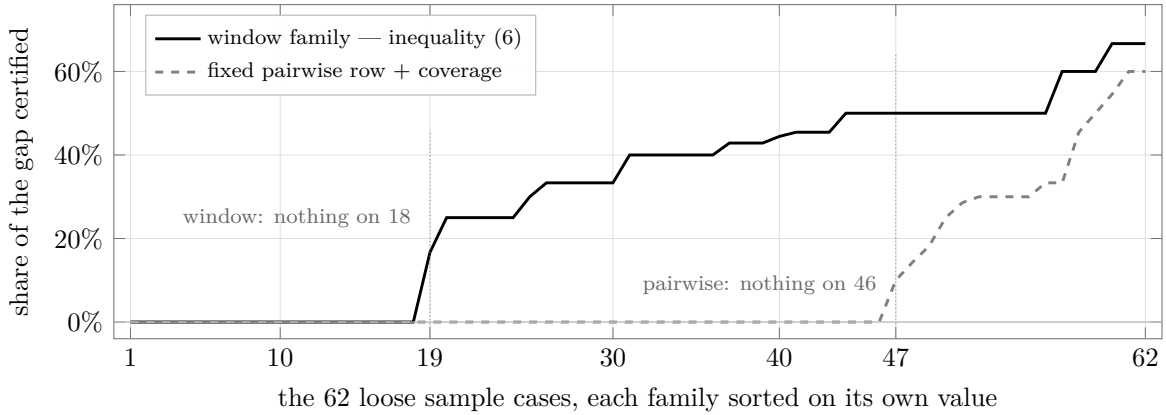
Figure 13: The integral-sequence value of each construction on each of the 62 loose sample cases, each sorted independently, so the curves answer how often does this construction certify anything, and how much . Each is the fraction of that instance’s gap closed after enumerating every ordering. The fixed pairwise row plus coverage is flat at zero for the first 46 instances and only then rises. This statement does not extend to all arc-supported cuts; the campaign-root cross-check in Table 12 shows why. The window family is flat at zero for 18 and then climbs, with its longest flat stretch at one half — 13 of the 62 instances — and only three reaching two thirds. The two peaks are similar, 60% against 67%, so the difference between the constructions lies in how often each certifies anything at all, rather than in how much it certifies when it does.
