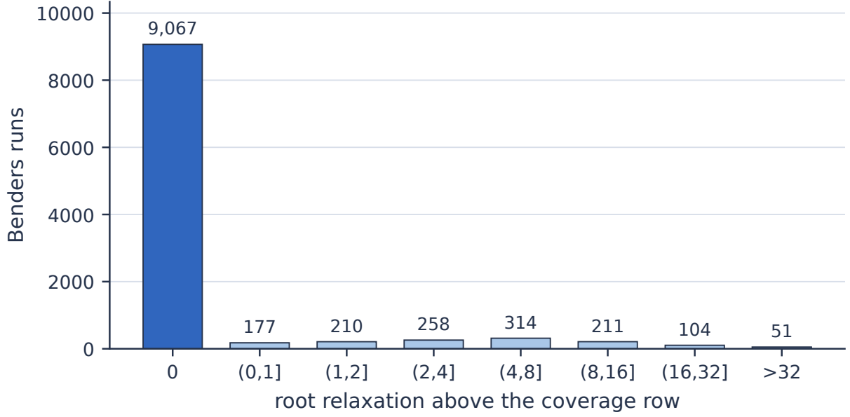
Figure 12: Observation 10 drawn over all 10,392 canonical Benders runs that recorded a root relaxation. The first bar is every run whose root value is exactly the coverage row — 9,067 of them, nearly seven times the whole remainder combined. The pairwise row, the triplet rows and every optimality cut generated before the first branching decision, taken together, move the relaxation not at all on eighty-seven runs in a hundred. This is the diagnosis behind the rest of this section stated as a single measurement. The master has no shortage of cuts; it is carrying one constant row and getting nothing from the others.
