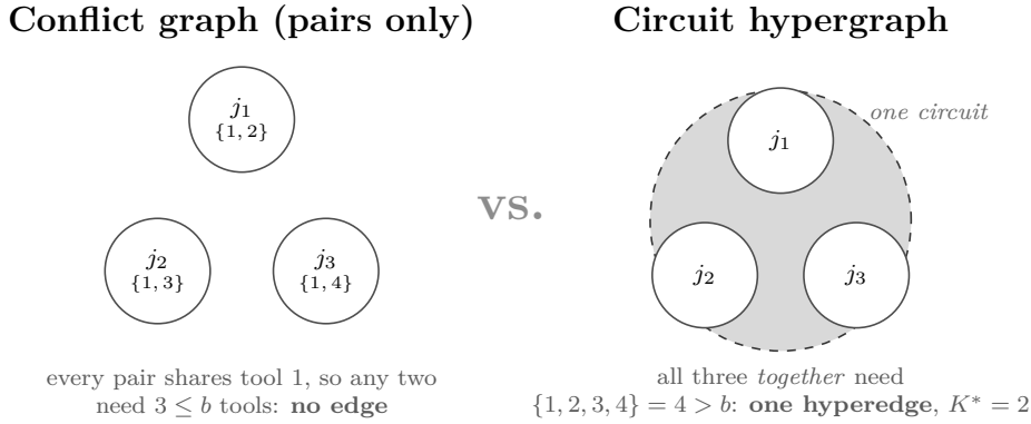
Figure 8: Why K^* is read off the hypergraph of all minimal clashes and never off the graph of pairwise ones. On this instance no two jobs conflict, because any two of them need only three tools, which fit. All three together need four and overflow the magazine, so they form a circuit, and that single circuit already forces two groups.
