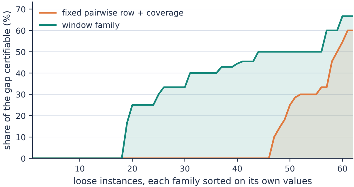
Figure 13: The integral-sequence value of each construction on each of the 62 loose sample cases, each sorted independently, so the curves answer how often does this construction certify anything, and how much . Each is the fraction of that instance’s gap closed after enumerating every ordering. The fixed pairwise row plus coverage is flat at zero for the first 46 instances and only then rises. This statement does not extend to all arc-supported cuts; the campaign-root cross-check in Table 12 shows why. The window family is flat at zero for 18 and then climbs, with its longest flat stretch at one half — 13 of the 62 instances — and only three reaching two thirds. The two peaks are similar, 60% against 67%, so the difference between the constructions lies in how often each certifies anything at all, rather than in how much it certifies when it does.
