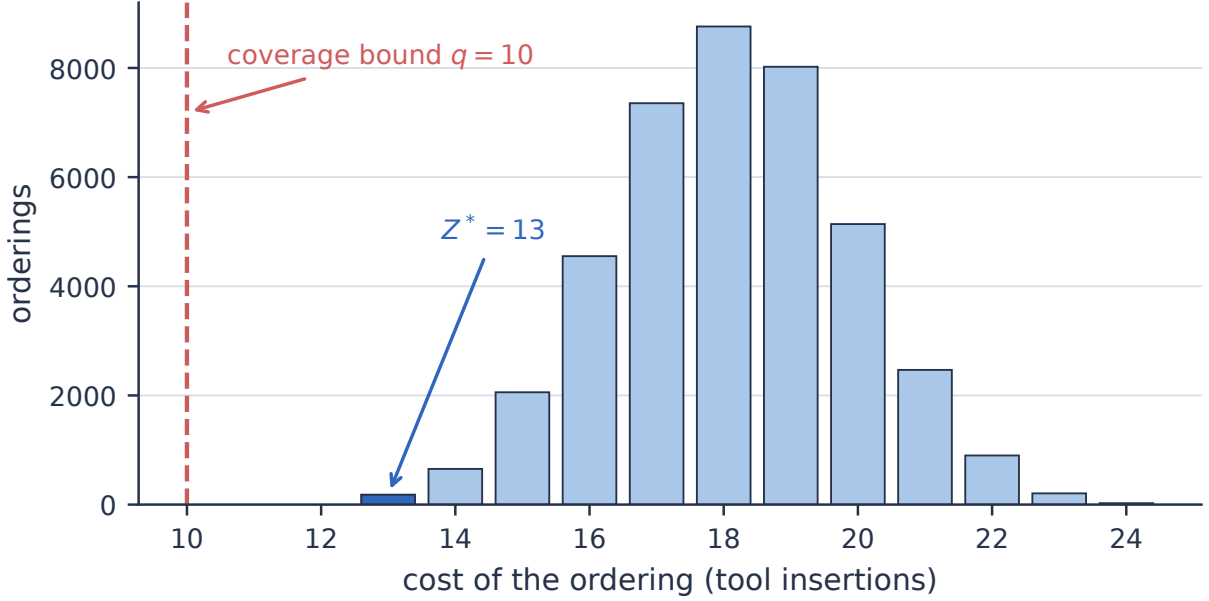
Figure 3: Every one of the 40,320 orderings of instance L1-1 ( n = 8 jobs, |U| = 15 tools, magazine b = 5 ), enumerated, and the tool switches each requires. Three things are visible at once. A randomly chosen ordering costs 18, and the best costs 13, so the choice of order is worth about a third of the total. Only 180 orderings out of forty thousand are optimal, which is why the outer problem is hard. And the counting bound of q = 10 , which is what the SSPMF compact baseline returns, lies below the entire distribution : no ordering whatsoever attains it. A solver given that bound cannot prove any ordering optimal until it has closed a gap of three by branching alone. Section 6 shows what that costs in practice and Section 7 why the bound behaves this way.
