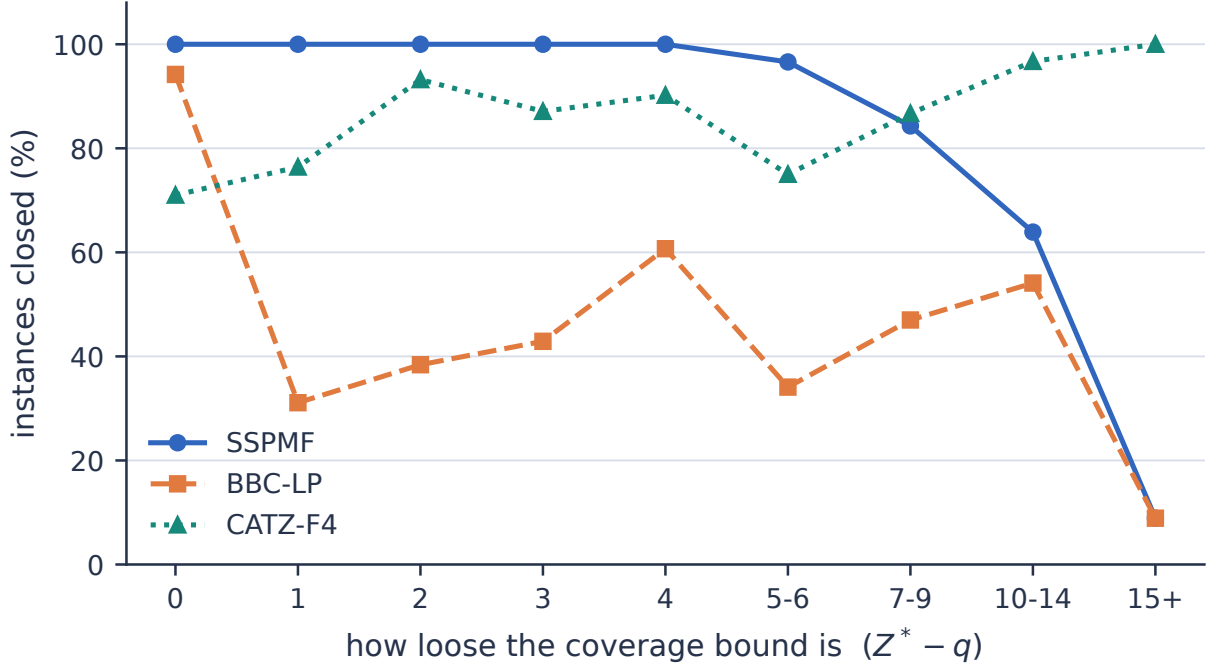
Figure 11: The 1,107 instances of known optimum, grouped by how far the optimum exceeds the coverage bound, against the share each method closes. Every bucket uses its full class size, with every non-optimal outcome counted as not closed. This is Table 10 resolved into its whole response curve, and the curve says more than the two-way split does. The Benders solver does not degrade: it falls off a cliff between a bound that is exact and a bound that is wrong by one, from 94% to 31%, and then wanders without trend — once the bound is loose at all, by how much stops mattering. SSPMF degrades smoothly instead, holding 100% out to a gap of four and then falling away, and it meets the Benders solver at the right-hand end: on the 45 instances whose bound is loose by fifteen or more, both close 8.9% — four each. CATZ-F4 does neither. Its curve rises, and on those same 45 instances it closes all 45, at a median of 93 seconds. Whatever makes the right-hand end hard is therefore not a property of those instances.
