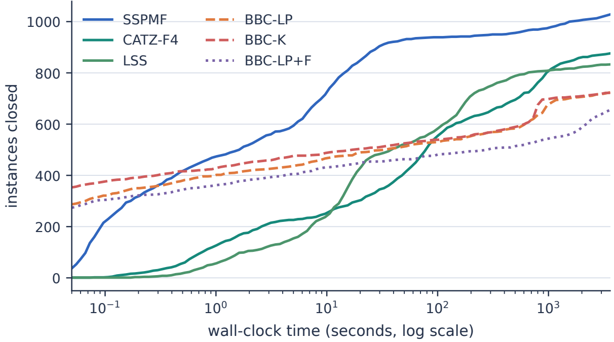
Figure 10: Every solved run in the campaign, not the six sampled columns of Table 8: for each method, the number of instances closed by each wall-clock time. What separates the two groups is not where they end but how they get there. Within one second the Benders configurations have closed between 55% and 60% of everything they will close in the hour, against 46% for SSPMF, 15% for CATZ-F4 and 7% for LSS: BBC-K has a median solve time of 0.06 seconds against 59.4 for CATZ-F4, because a master with a tight coverage row closes an instance at the root almost at once or does not close it at all. In absolute counts that lead is brief — SSPMF passes every Benders configuration at about half a second and is never caught, while BBC-K stays ahead of LSS until about a minute and BBC-LP ahead of CATZ-F4 until about 87 seconds. No curve has stopped when the limit arrives: over the last decade of the axis BBC-LP still gains 154 instances and CATZ-F4 210, against 78 for SSPMF, which is the method nearest to saturation. A longer limit would therefore move the counts, and not equally.
