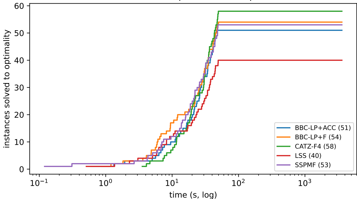
Performance profile (cactus plot)
