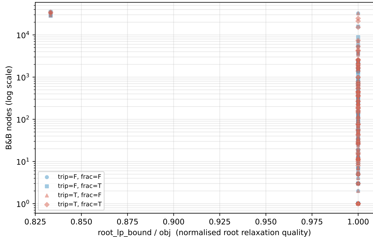
Root LP Bound Quality vs. B&B Tree Size (BBC configs, primary instances)
