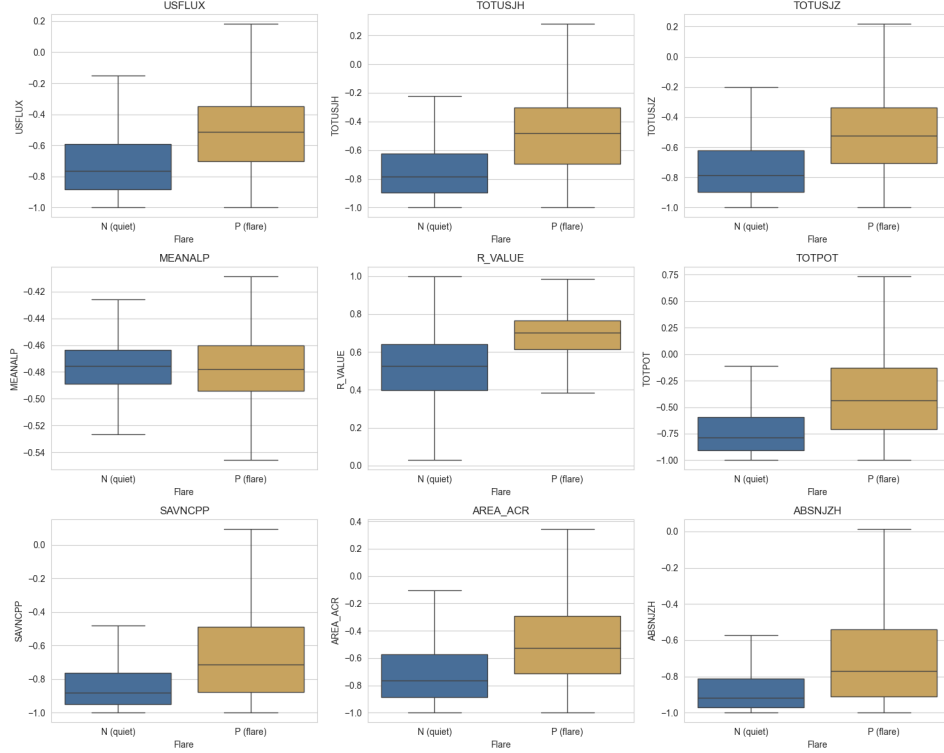
Figure 3: Feature distributions split by class (N = quiet, P = flare).
