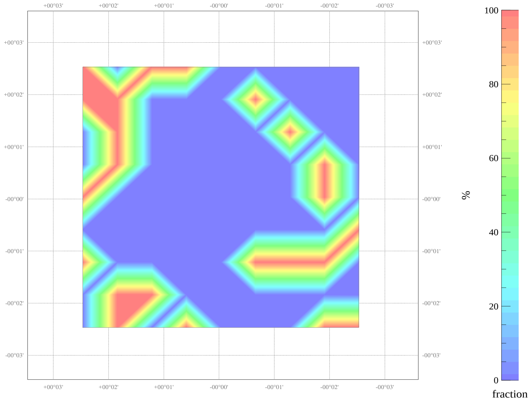
Field NGC_3245: source count fraction map
