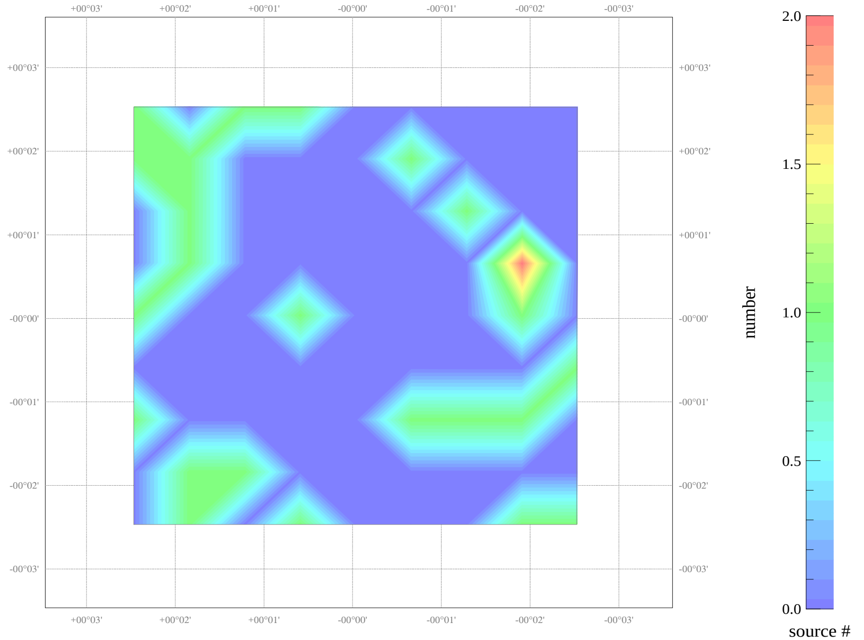
Field NGC_3245: source count map
