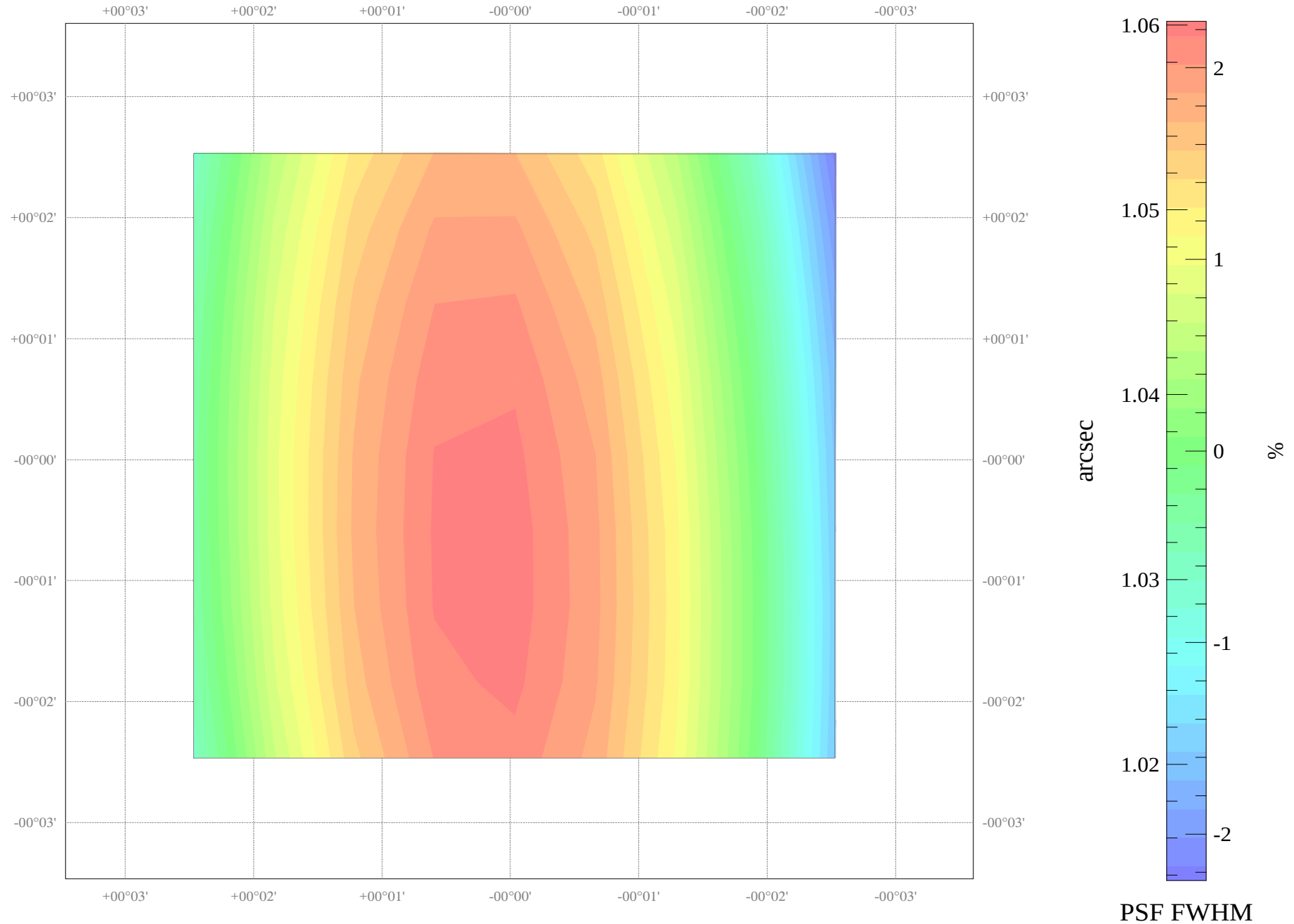
Field NGC_3245: FWHM map
