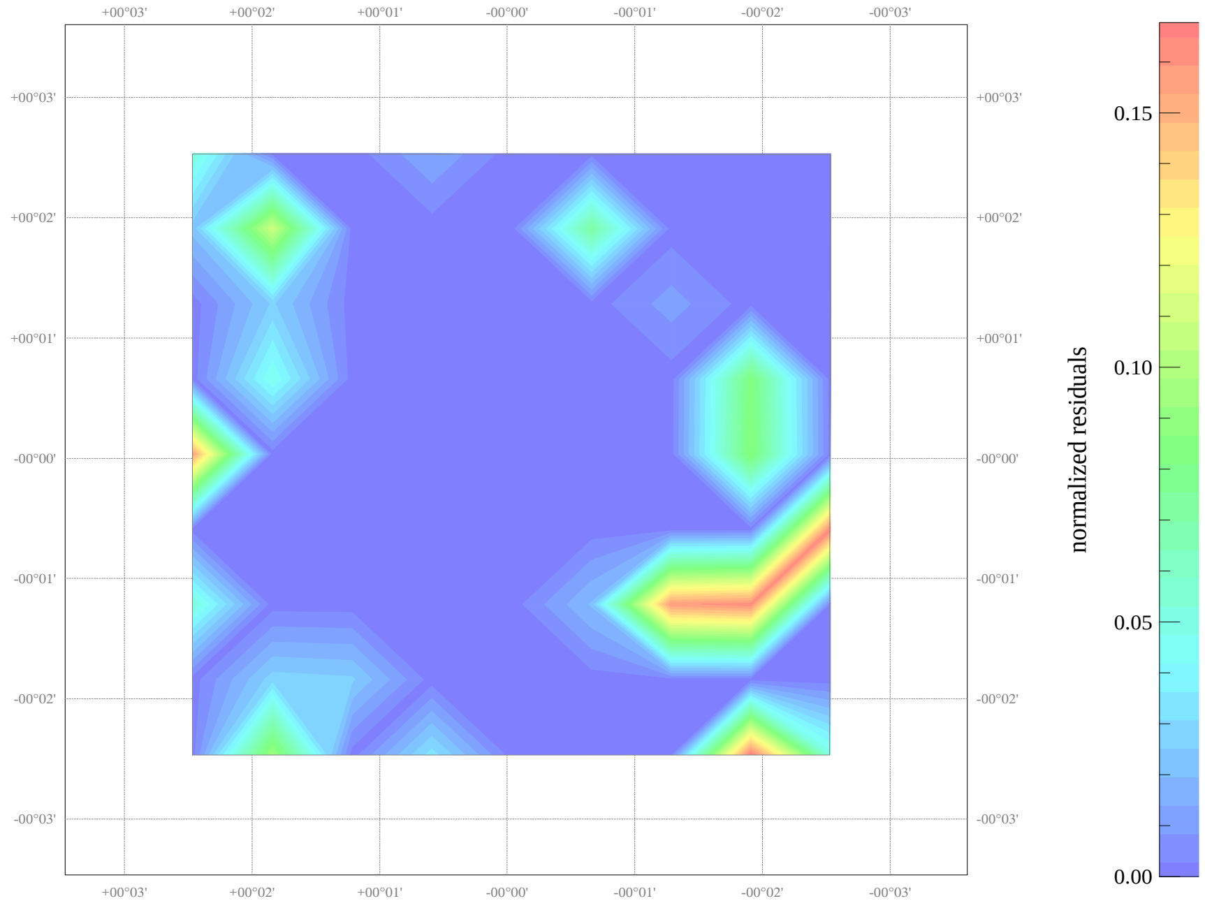
Field NGC_3245: map of residuals
