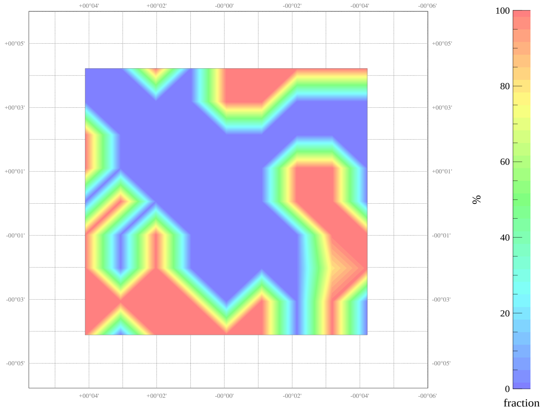
Field NGC_3938: source count fraction map
