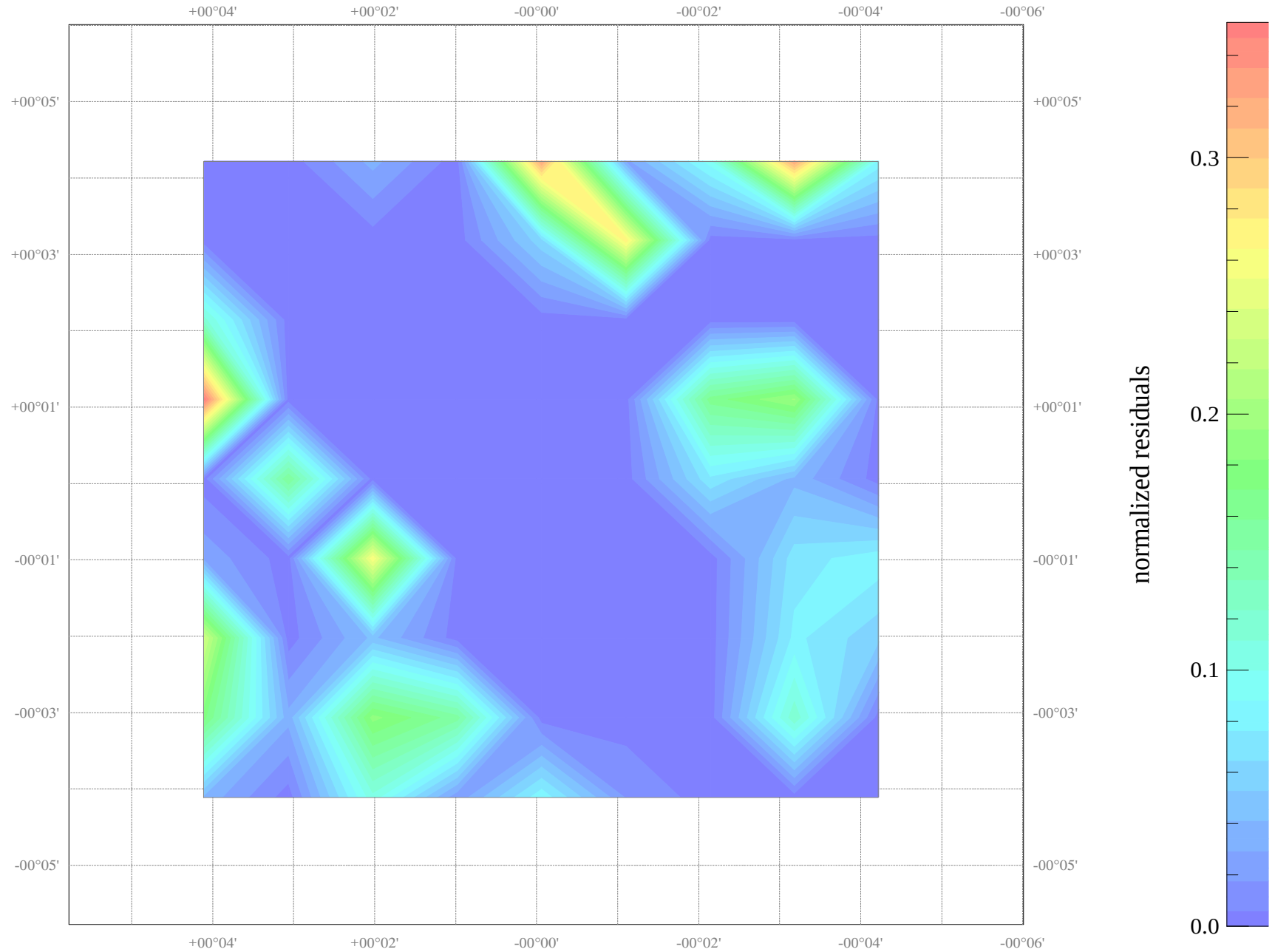
Field NGC_3938: map of residuals
