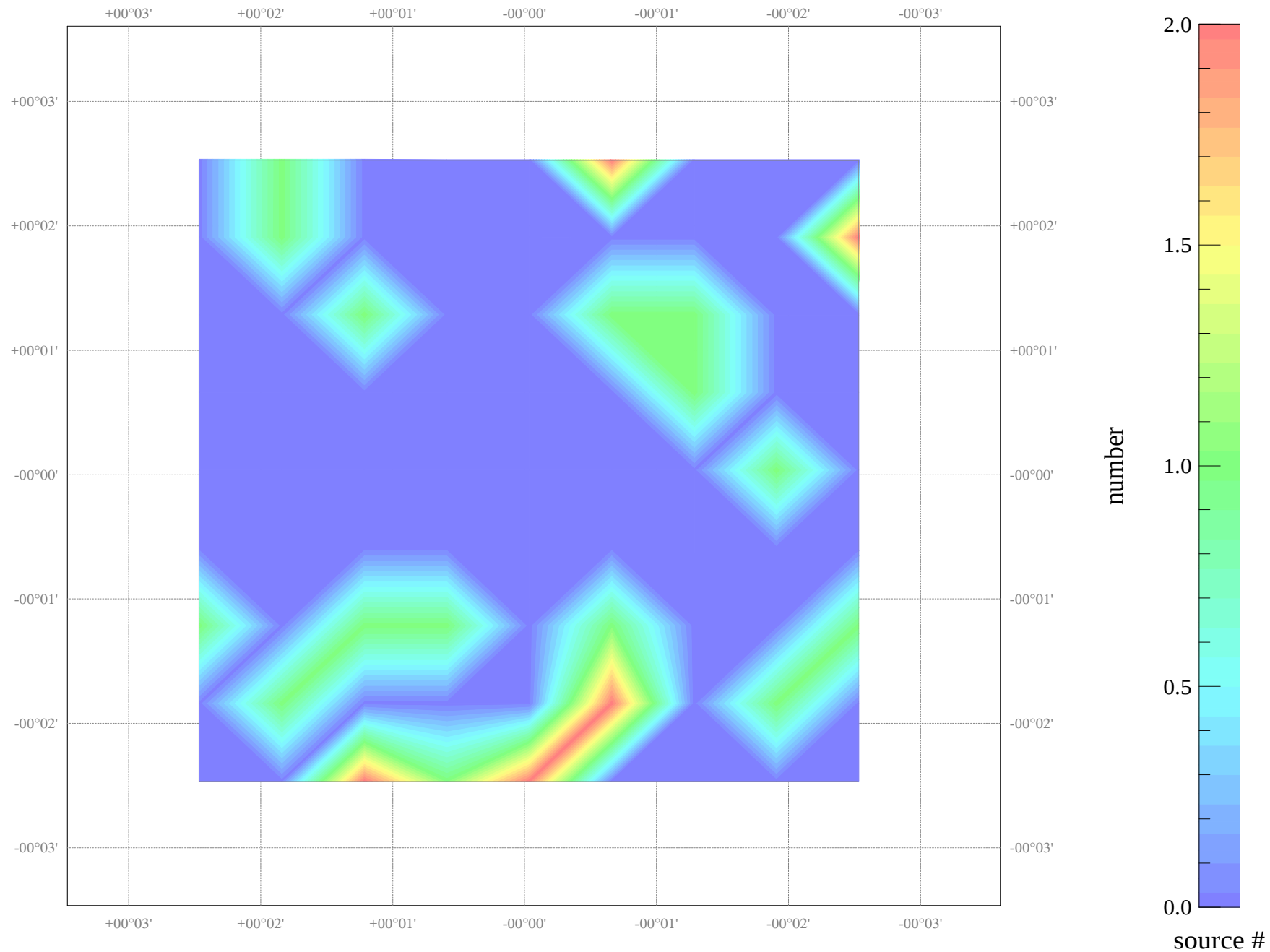
Field NGC_4378: source count map
