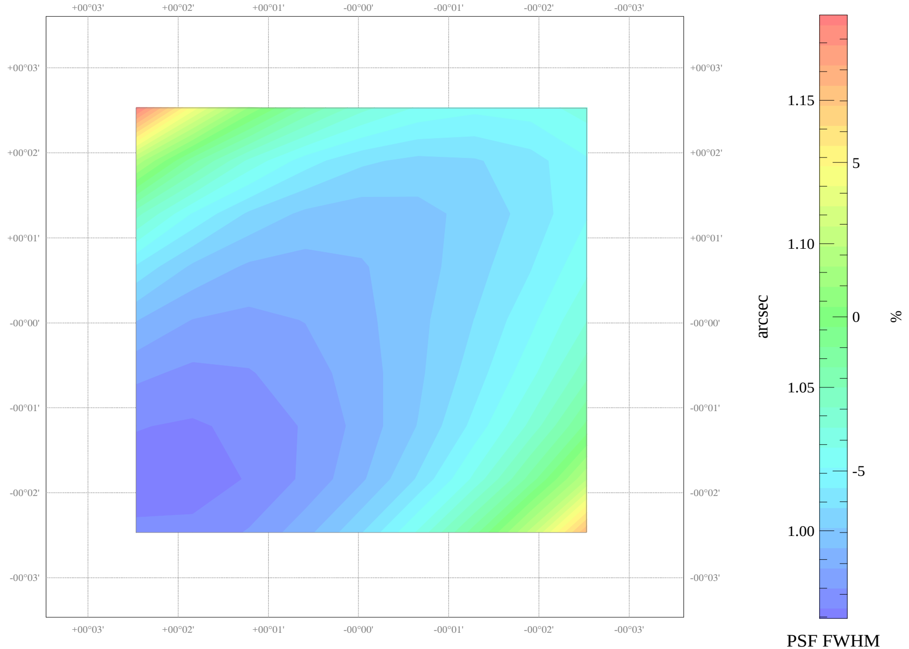
Field NGC_4378: FWHM map
