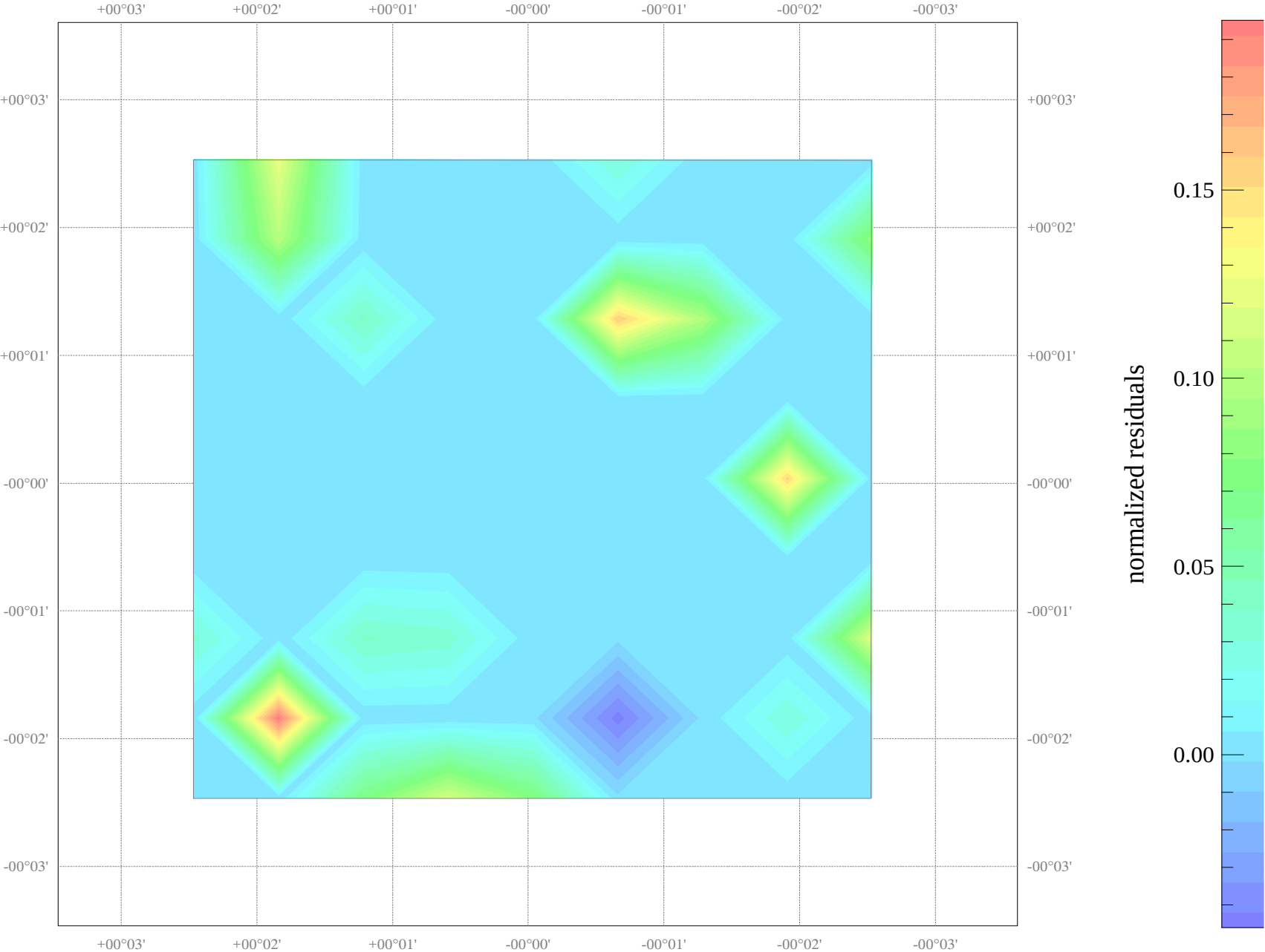
Field NGC_4378: map of residuals
