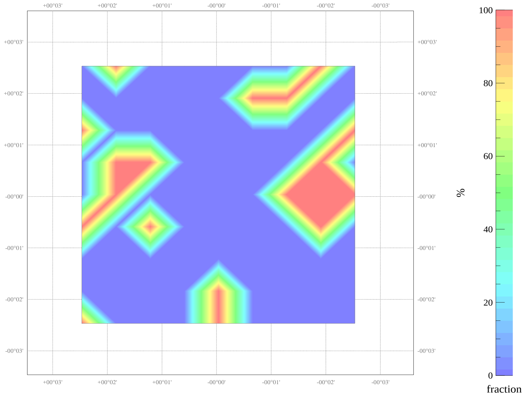
Field NGC_4623: source count fraction map
