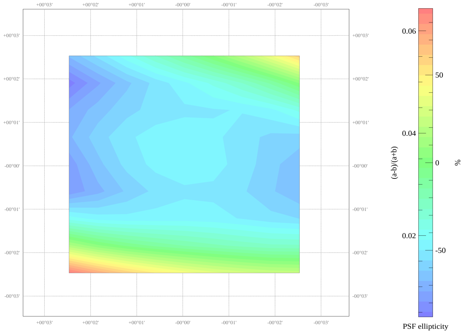
Field NGC_4623: ellipticity map
