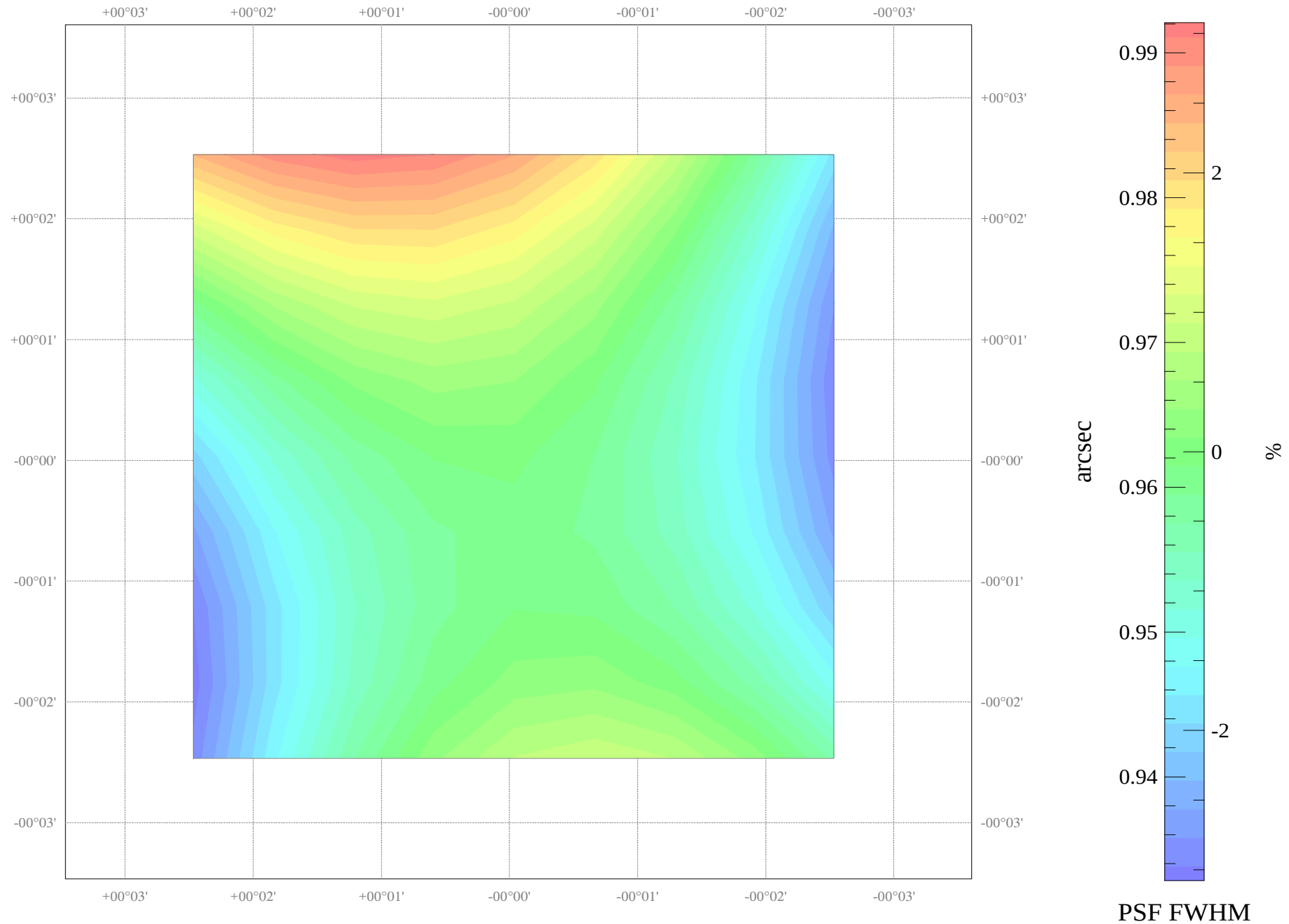
Field NGC_4623: FWHM map
