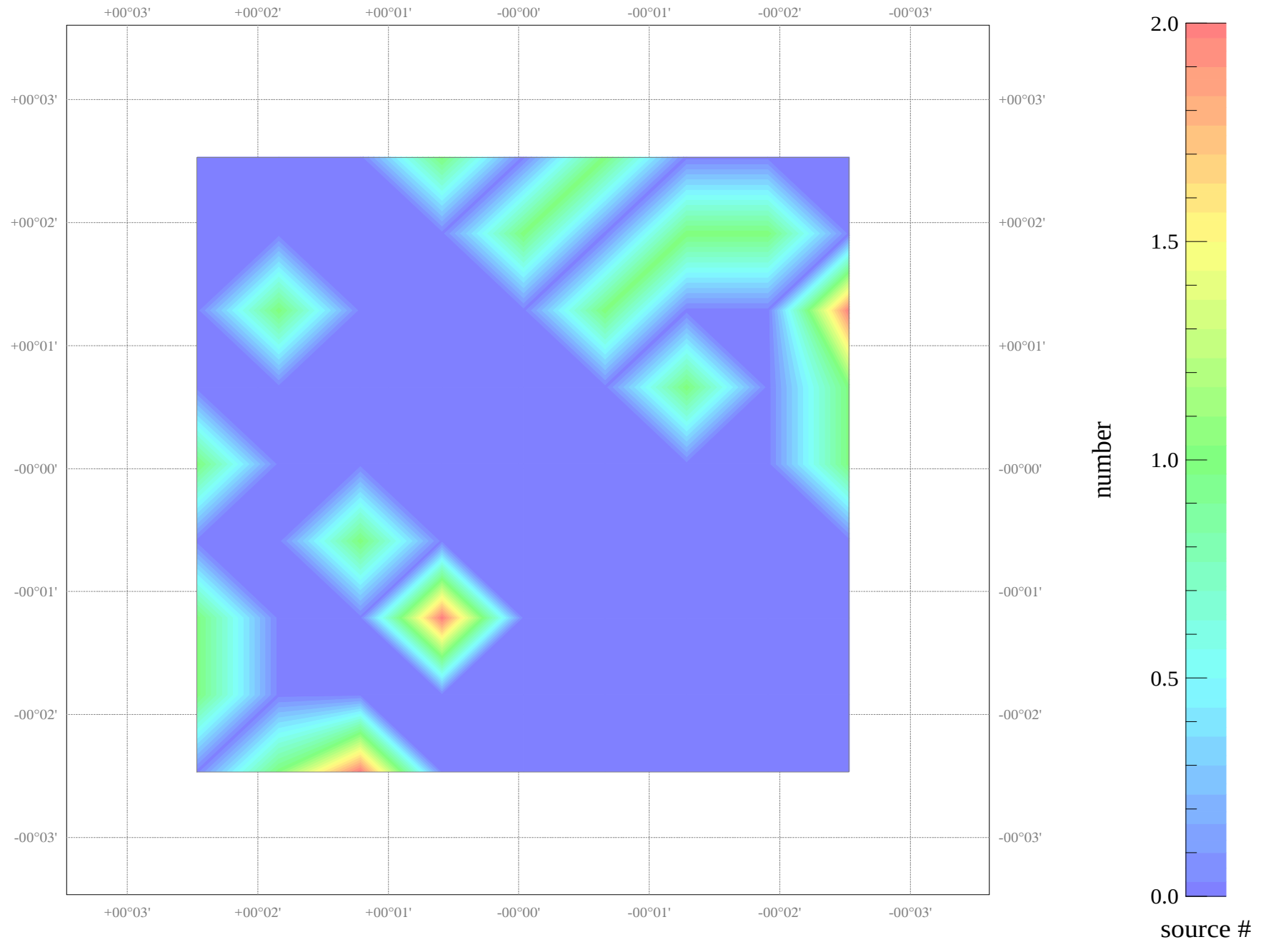
Field NGC_4762: source count map
