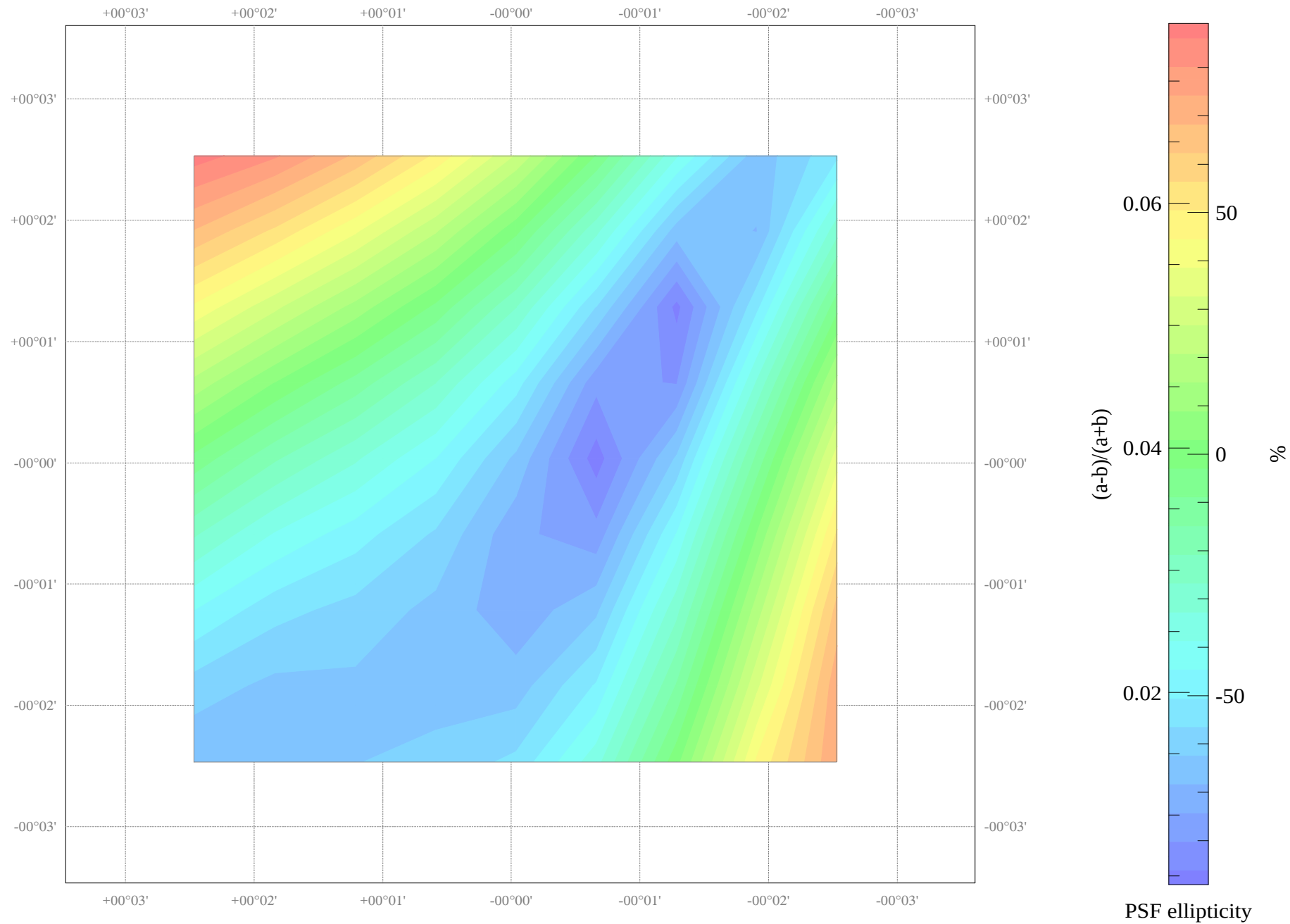
Field NGC_4762: ellipticity map
