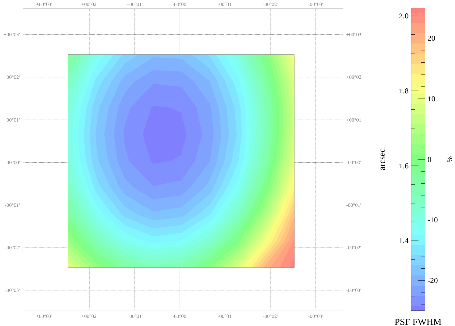
Field NGC_4762: FWHM map
