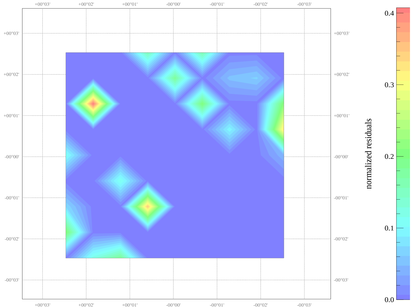
Field NGC_4762: map of residuals
