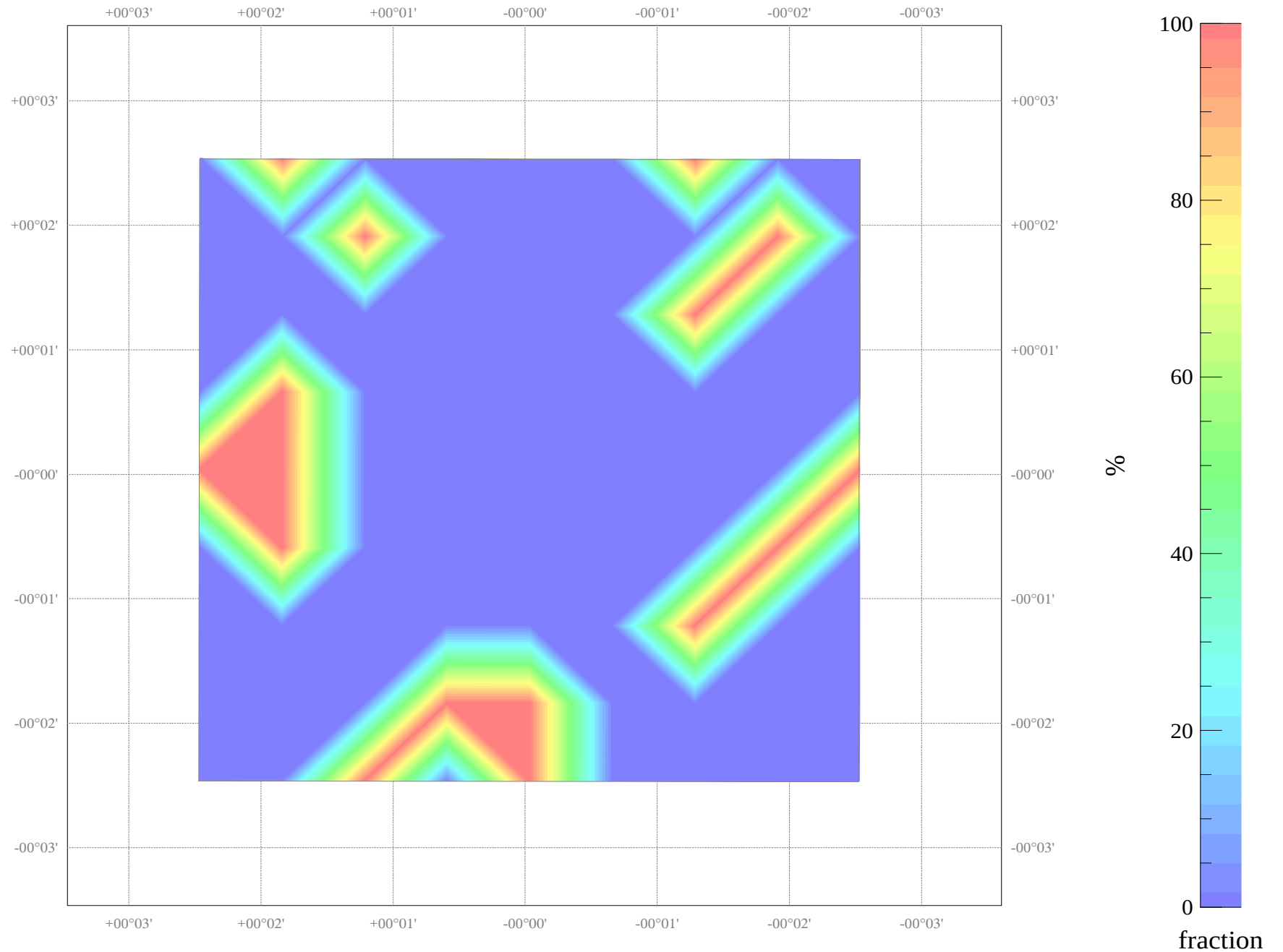
Field NGC_4814: source count fraction map
