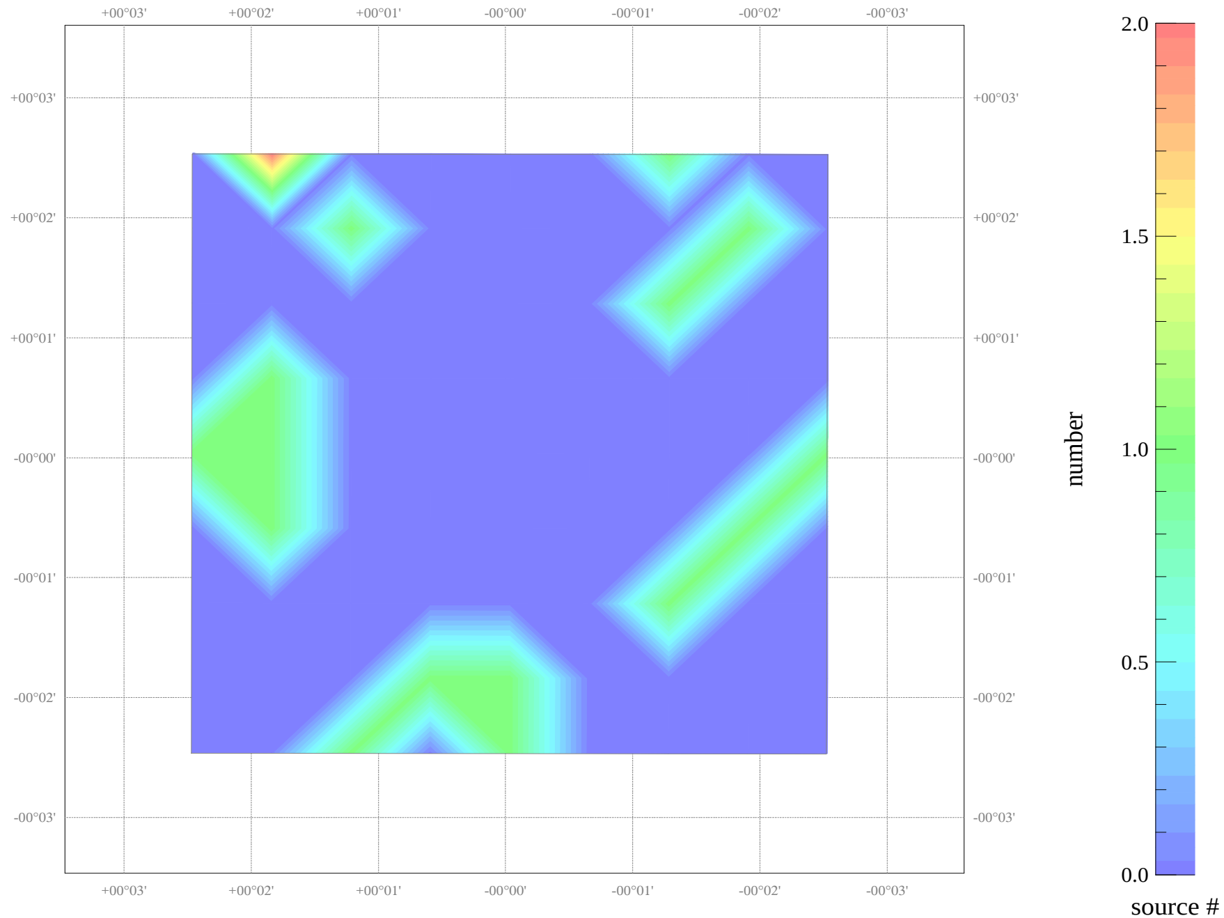
Field NGC_4814: source count map
