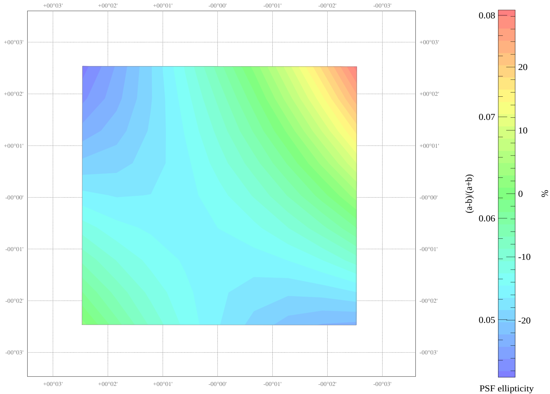
Field NGC_4814: ellipticity map
