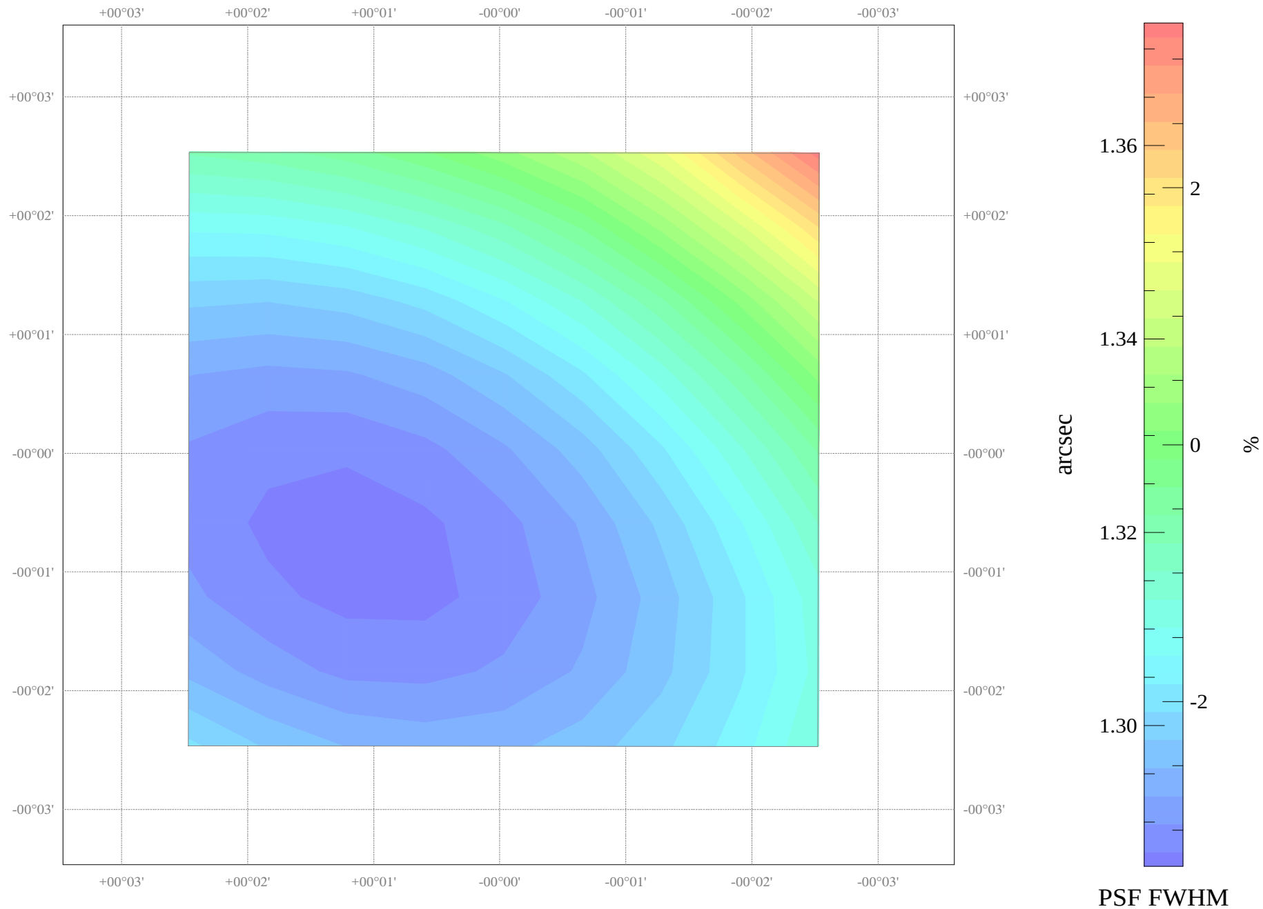
Field NGC_4814: FWHM map
