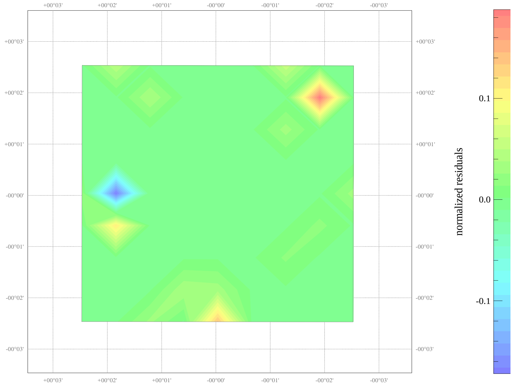
Field NGC_4814: map of residuals
