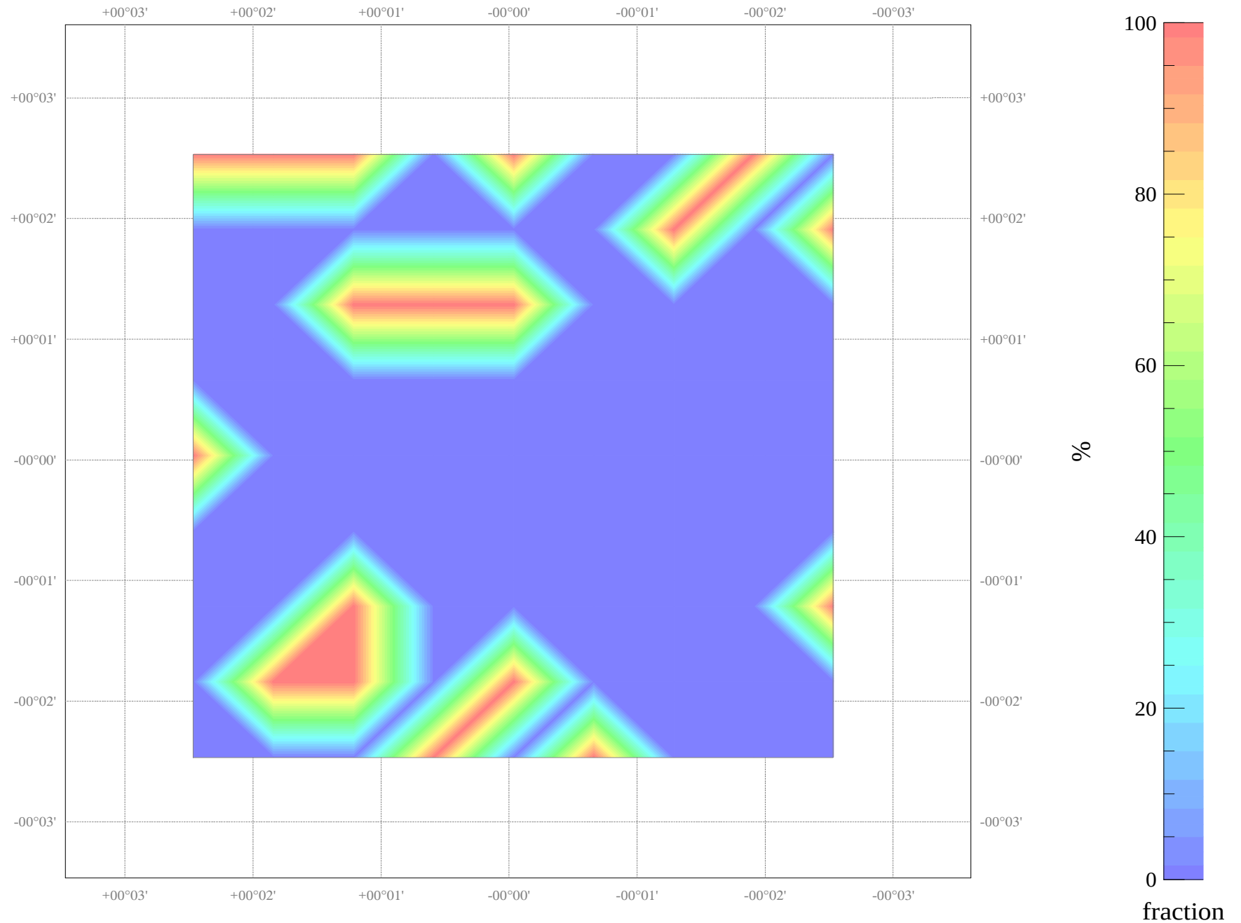
Field NGC_5576: source count fraction map
