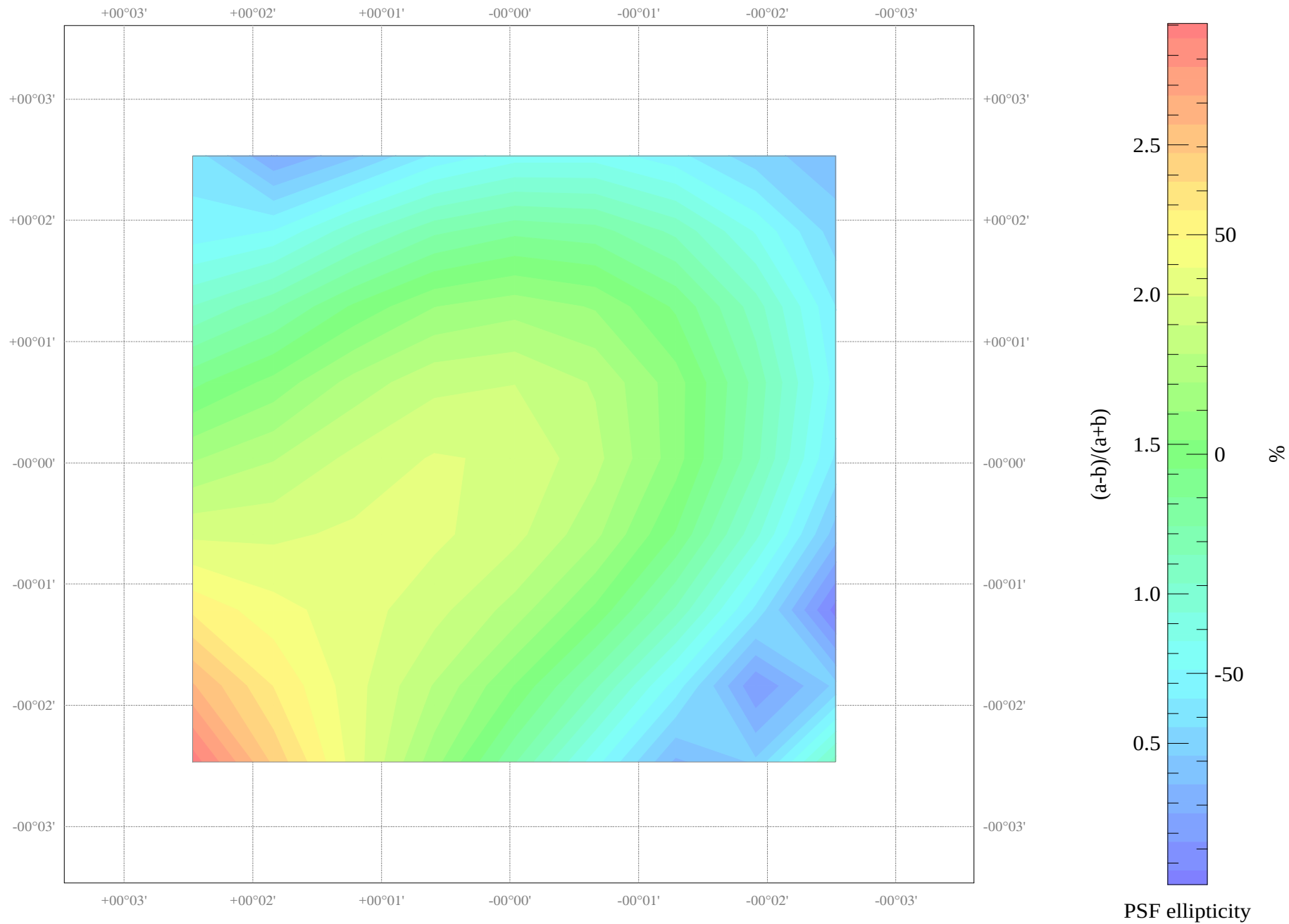
Field NGC_5576: ellipticity map
