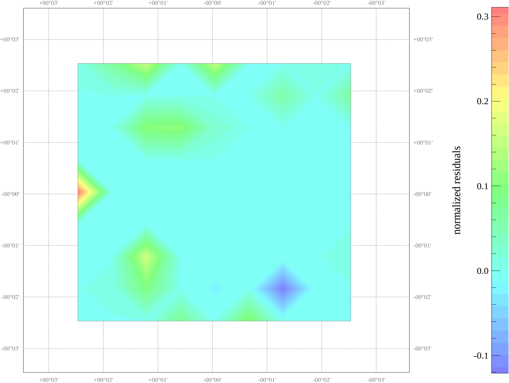
Field NGC_5576: map of residuals
